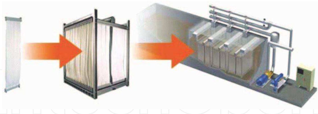
Fig. 8. Submerged membrane module for wastewater treatment. From ZeeWeed® Submerged Membrane System, from http://www.gewater.com .
