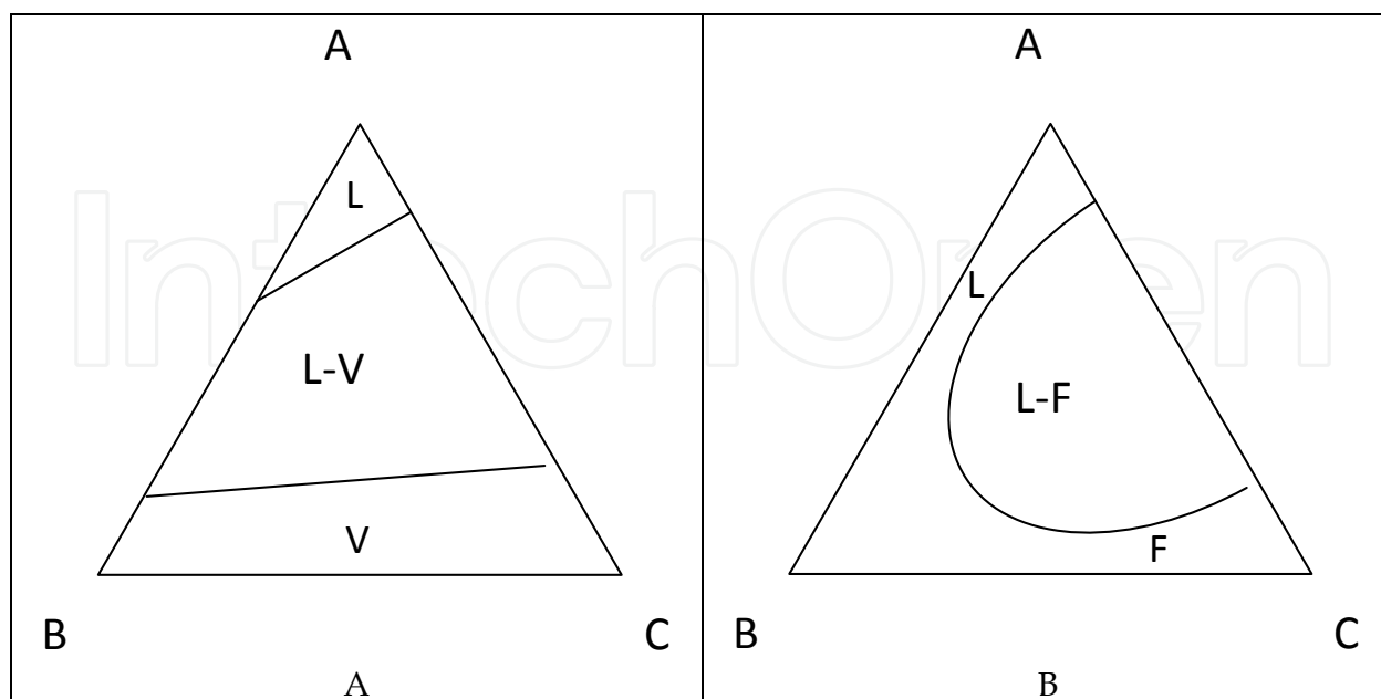
A: Vapor-Liquid Equilibria (VLE), B: if T or P is increased a supercritical fluid (F) appears and so a FLE.
