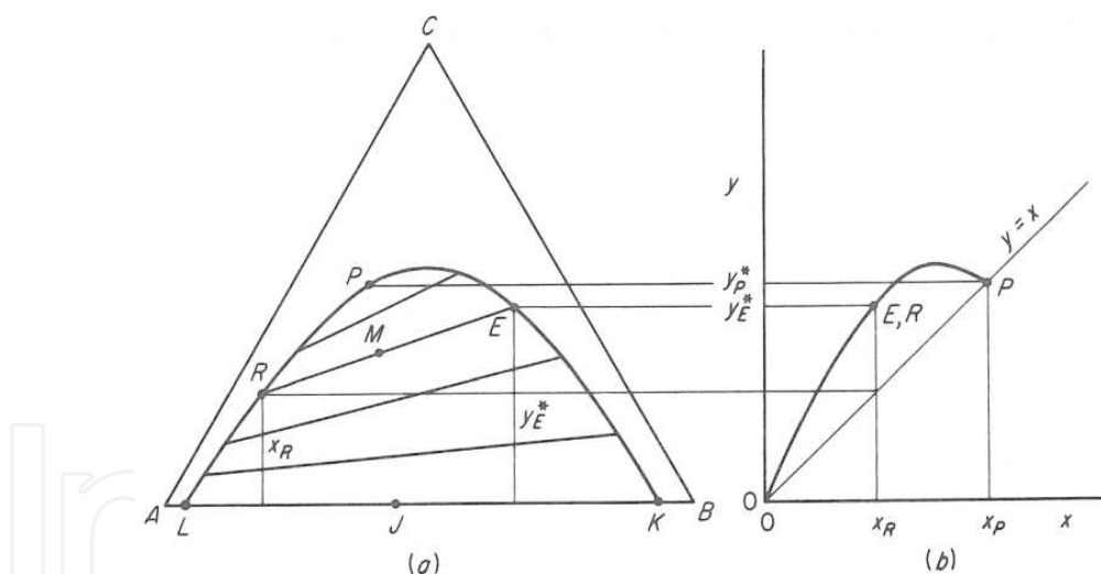
Fig. 17. Triangular (a) and distribution diagram (b) for liquid-liquid equilibria for a system of three components where one pair is partially miscible (extracted from Treybal, 1981).
