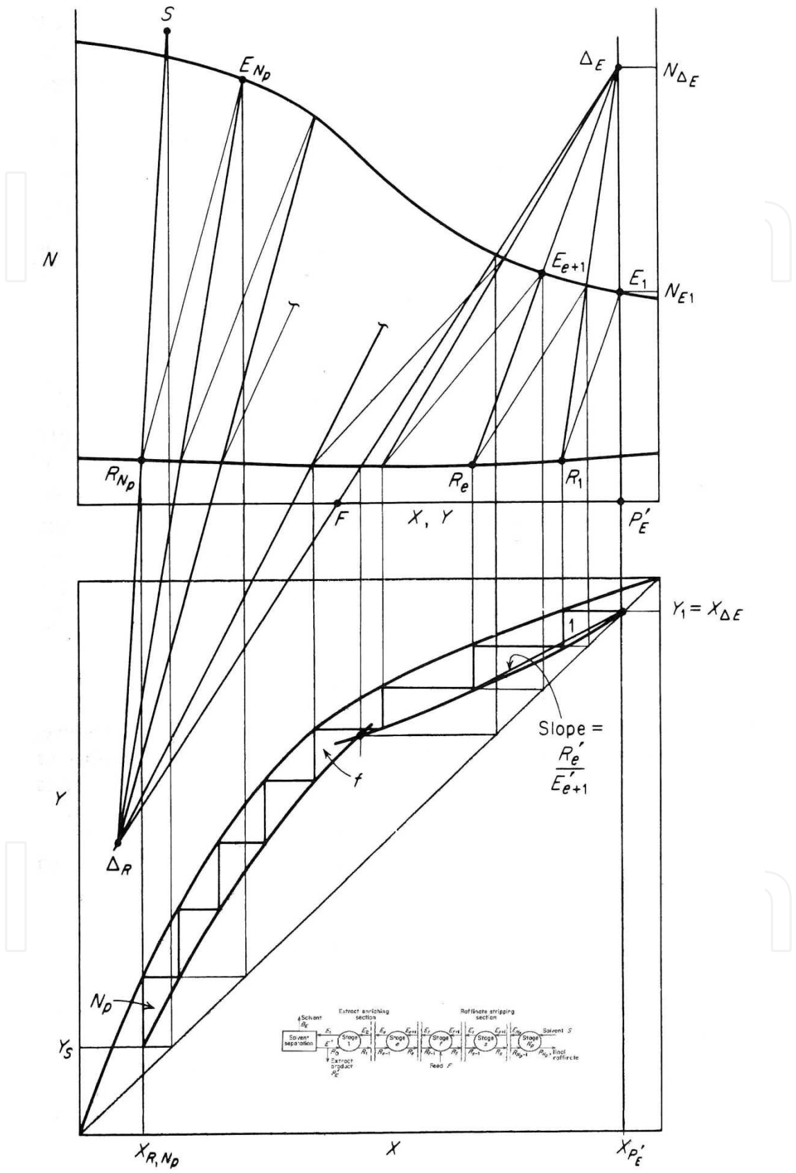
Fig. 18. Illustration of phase diagrams generated for a countercurrent extraction process with reflux (extracted from Treybal, 1981)
