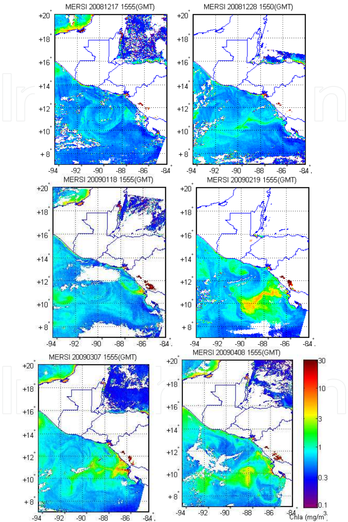
Fig. 7. Red tide process in Central America.
