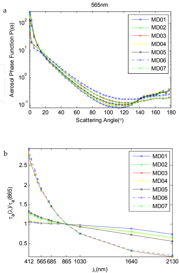
Fig. 5. Aerosol scattering phase function for 565nm band (a) and normalized aerosol optical thickness (b).
