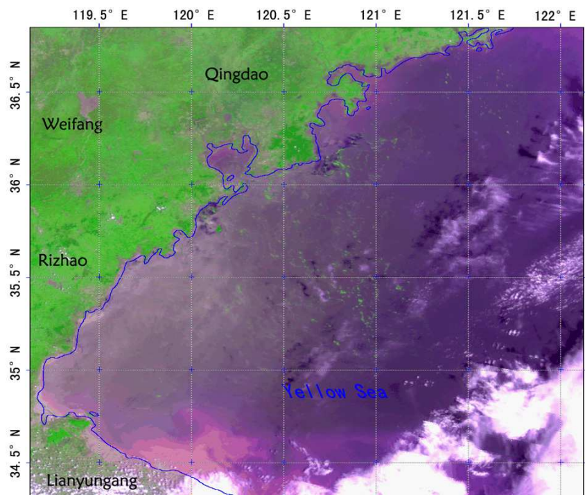
Fig. 6. Algae bloom captured on June 28, 2008 around Qingdao.
