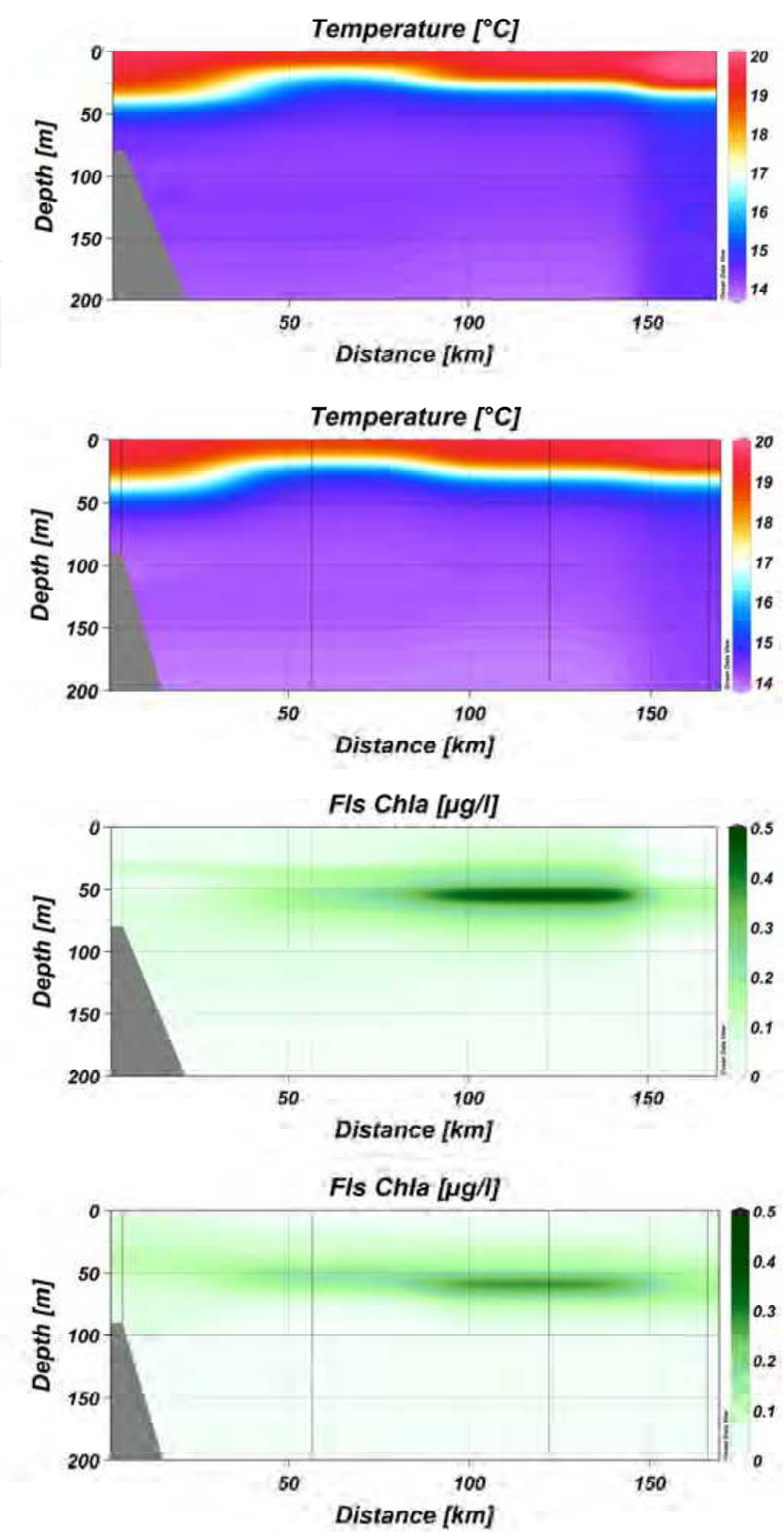
Fig. 13b. ADR0208 cruise: depth-distance sections (W-E oriented) obtained by means of T-FLAP and SBE 911 plus CTD-Chelsea Aquatraka fluorometer: temperature upside; fluorescence downside (data analysed with ODV - Schlitzer, 2011)
