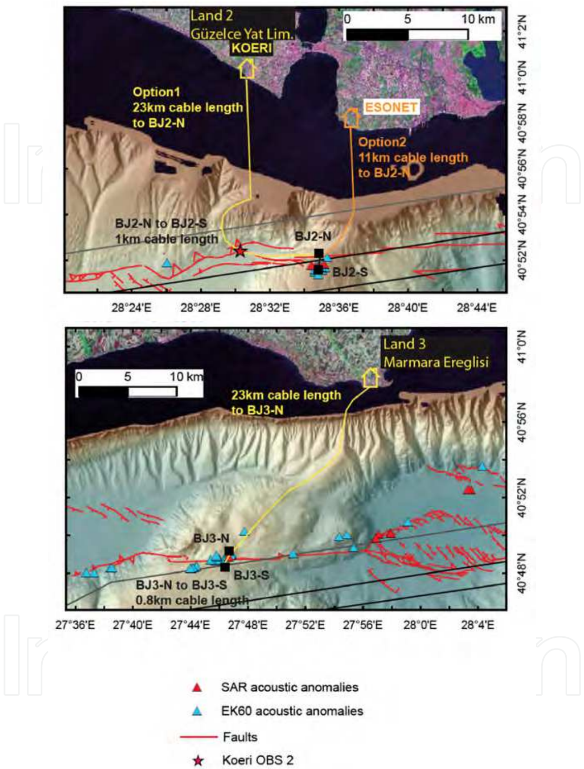
Fig. 22. View of the cable (yellow line) linking the observatory to the node at P1 (lower figure) and P2 (upper figure). The cable will be deeply buried all the way from shore to the main node. The area between the two SW-NE oriented, black lines is the separation zone between the upgoing and downgoing navigation corridor. The northern limit of the downgoing corridor is indicated as a thin grey line. The red star indicates the planned location of a cabled, permanent OBS to be deployed by KOERI in 2011.
