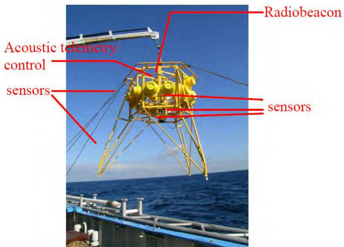
Fig. 1. BOBO lander in previous version (source: http://mars-srv.oceanlab.iu-bremen.de/infra_obser_bobo.html )
