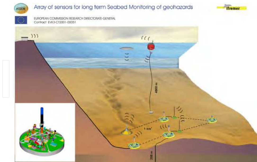
Fig. 5. An ASSEM node and a sketch of multi ASSEM node system ©Ifremer
