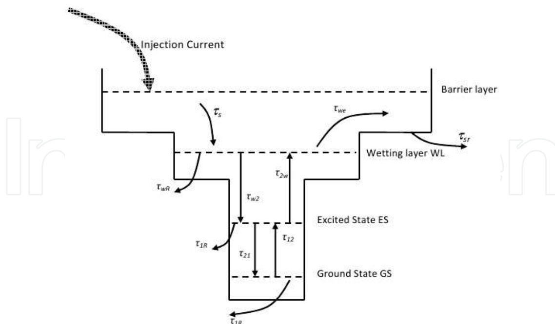
Fig. 2. Energy diagram of QD-SOA system.
