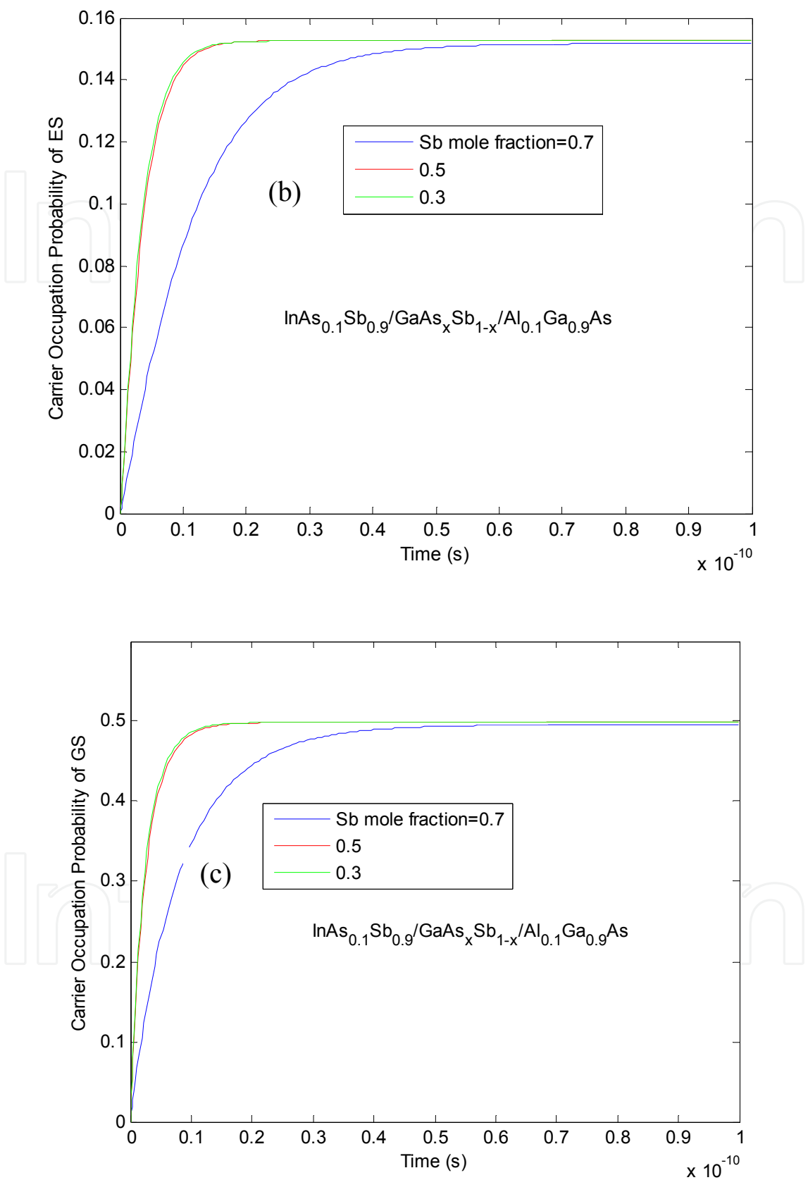
Fig. 6. (a) Carrier density for WL. Then occupation probability for: (b) ES and (c) GS for \text{InAs}_{0.1}\text{Sb}_{0.9}/\text{GaAs}_x\text{Sb}_{1-x}/\text{Al}_{0.1}\text{Ga}_{0.9}\text{As} QD-SOAs
