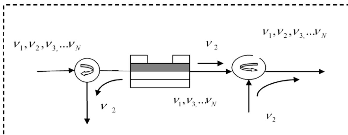
Fig. 1(b). SOA based add/drop multiplexer
