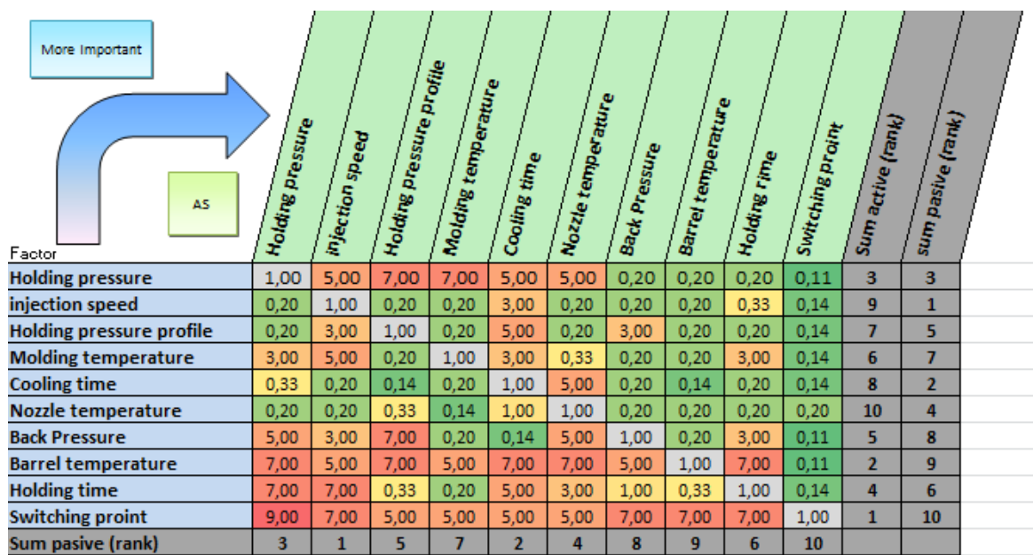
Fig. 4. AHP Matrix 2 .
