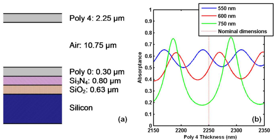
Fig. 6. (a) Schematic of a SUMMiT V TM polysilicon MEMS structure and (b) its optical response at different wavelengths as a function of the thickness of the top-most layer. The variation in the amplitude and width of the absorptance peaks in this structure is related to the relative reflectivity of the two polysilicon surfaces at the particular wavelength much like a Fabry-Perot cavity (Born & Wolf, 1999) and will ultimately depend on the overall composition of the multilayered structure. For a coupled optical-thermal analysis, the existence of these periodic variations in the absorptance must be taken into account to predict the thermal behavior of laser-irradiated MEMS accurately.
