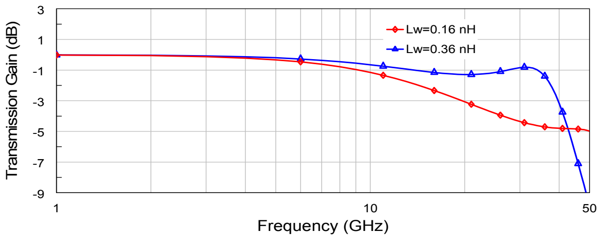
Fig. 9. The photodiode packaging effect simulation
