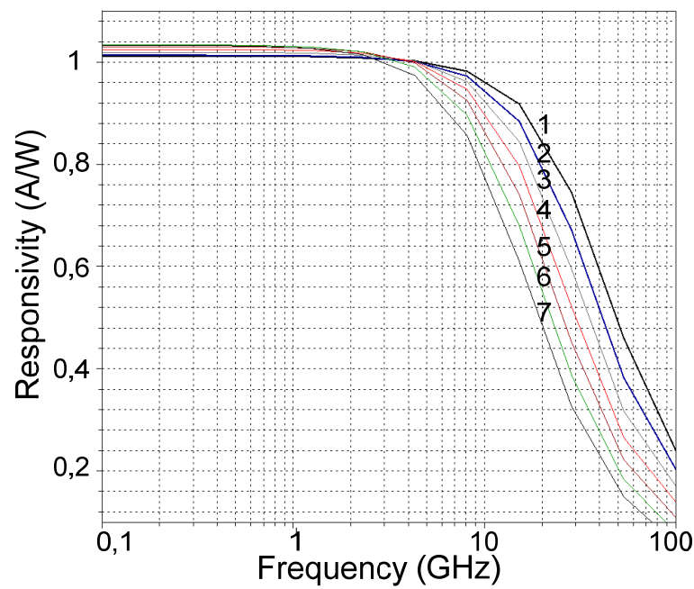
Fig. 7. The bandwidth vs. photosensitive window width simulation for a usual top-illuminated p-i-n photodiode structure with single heterojunction (1: w=18\text{ }\mu\text{m} ; 2: w=20\text{ }\mu\text{m} ; 3: w=22\text{ }\mu\text{m} ; 4: w=24\text{ }\mu\text{m} ; 5: w=26\text{ }\mu\text{m} ; 6: w=28\text{ }\mu\text{m} ; 7: w=30\text{ }\mu\text{m} )
