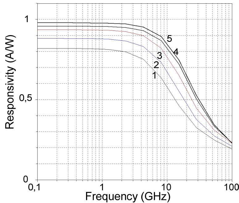
Fig. 5. The bandwidth vs. absorption region thickness simulation (1: s=0.3\text{ }\mu\text{m} ; 2: s=0.55\text{ }\mu\text{m} ; 3: s=0.8\text{ }\mu\text{m} ; 4: s=1\text{ }\mu\text{m} ; 5: s=1.3\text{ }\mu\text{m} )
