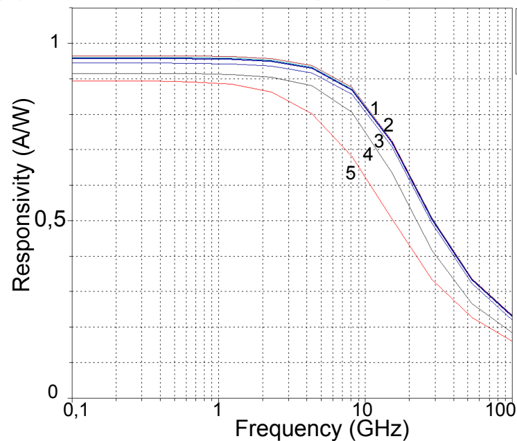
Fig. 4. The bandwidth vs. absorption region doping density simulation (1: N_D=8 \cdot 10^{15}\text{ cm}^{-3} ; 2: N_D=1 \cdot 10^{16}\text{ cm}^{-3} ; 3: N_D=2 \cdot 10^{16}\text{ cm}^{-3} ; 4: N_D=3 \cdot 10^{16}\text{ cm}^{-3} ; 5: N_D=4 \cdot 10^{16}\text{ cm}^{-3} )
