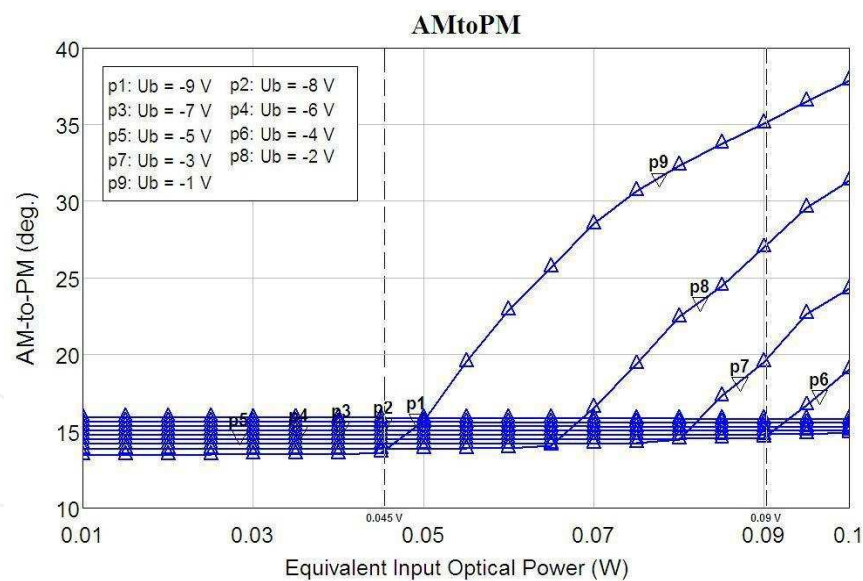
Fig. 12. Photodiode power to phase conversion characteristics
