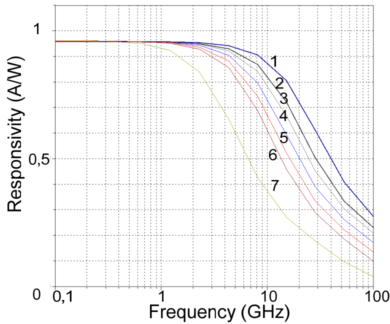
Fig. 6. The bandwidth vs. photosensitive window width simulation (1: w=18\text{ }\mu\text{m} ; 2: w=20\text{ }\mu\text{m} ; 3: w=22\text{ }\mu\text{m} ; 4: w=24\text{ }\mu\text{m} ; 5: w=26\text{ }\mu\text{m} ; 6: w=28\text{ }\mu\text{m} ; 7: w=30\text{ }\mu\text{m} )
