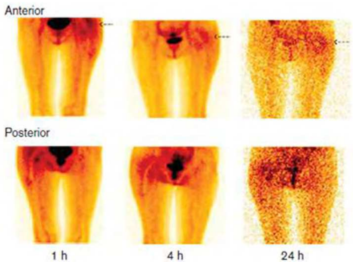
Fig. 4. 99mTc-Ciprofloxacin (Diagnobact™) scan (static anterior and posterior images) acquired at 1, 4 & 24h indicating increased radiotracer concentration in the region of left hip joint prosthetic (arrows)
