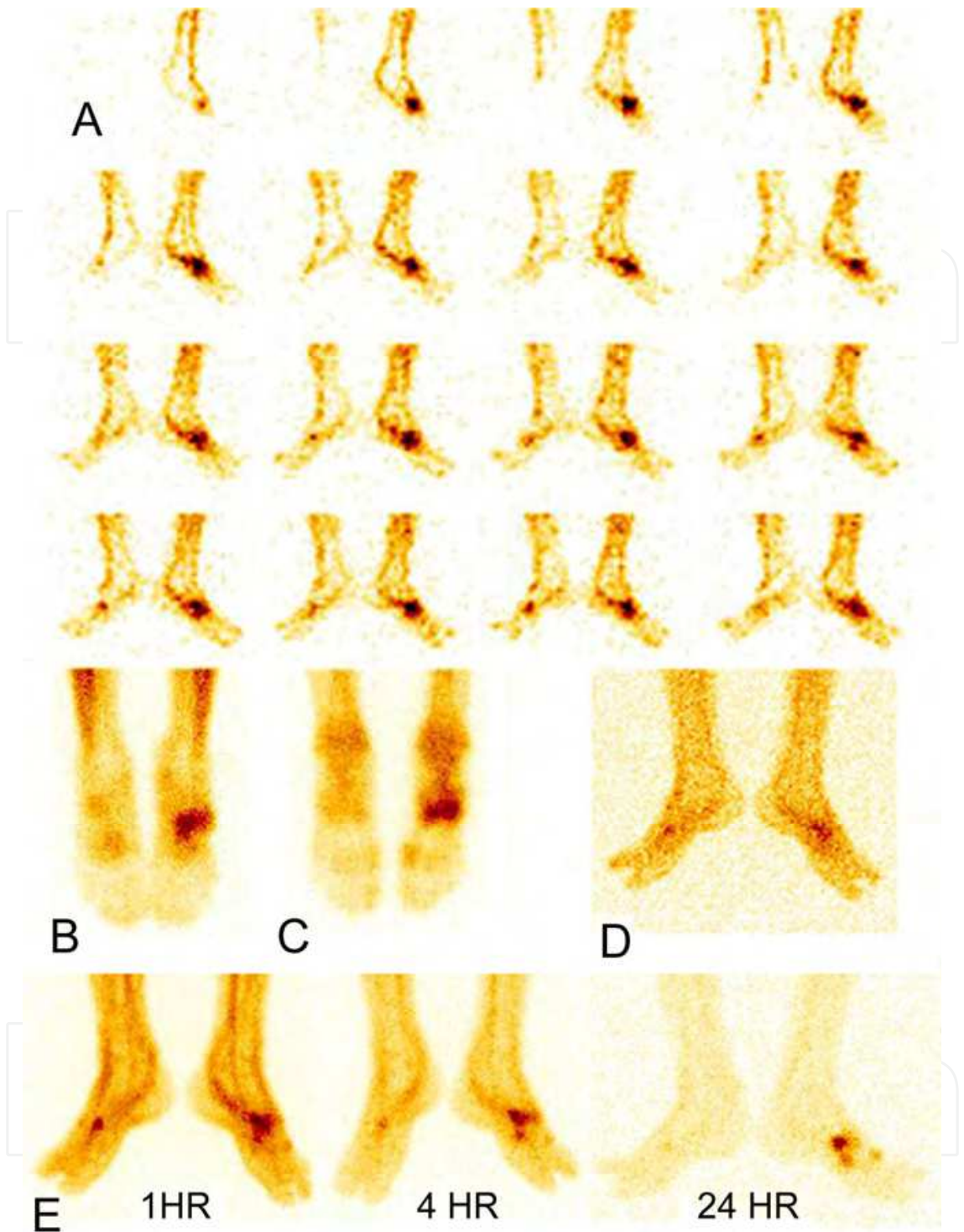
Fig. 3. Three phase bone scintigraphy of the feet with ^{99m}\text{Tc} -MDP showing increased flow (A) and soft tissue concentration (B) of tracer in the mid part of the left foot. The delayed images (C) at 3h shows focally increased bony uptake of tracer in the mid-tarsal region, indicating active bony infection. ^{99m}\text{Tc} -HMPAO labeled leukocyte images (E) at 1, 4, 24-h show focal tracer concentration in the mid-tarsal region of the left foot indicative of active infection. Bone marrow scan (D) performed 1-h after injection of 4.0 mCi of filtered ^{99m}\text{Tc} -Sulfo-colloid shows mild uptake in the mid-tarsal region less than ^{99m}\text{Tc} -MDP and labeled leukocyte uptake.
