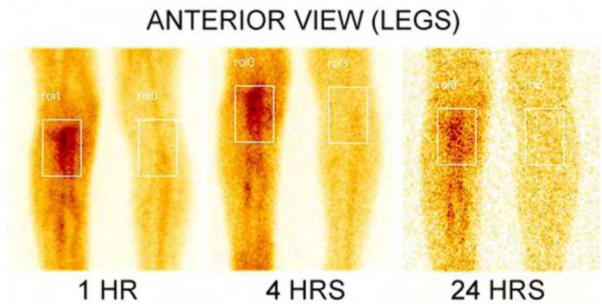
Fig. 5. 99mTc-Ceftriaxone (Scintibact) images of the legs showing focally increased concentration of the radiotracer in the proximal part of the right tibia. The radiotracer concentration remained consistent till 24-h of imaging time indicating active tibial infection
