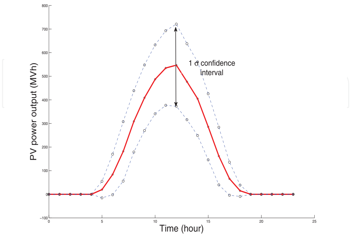
Fig. 14. Fluctuations in the output power of a large PV system (1σ confidence interval) (NSRDB, 2005)
