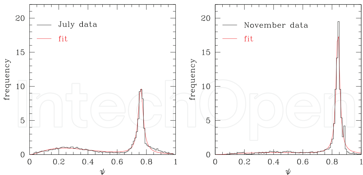
Fig. 13. The observed distribution of \psi and the two component fit for July ( left ) and November ( right ). Comparing both plots a shift in the centre of the narrow component is clearly appreciated.
