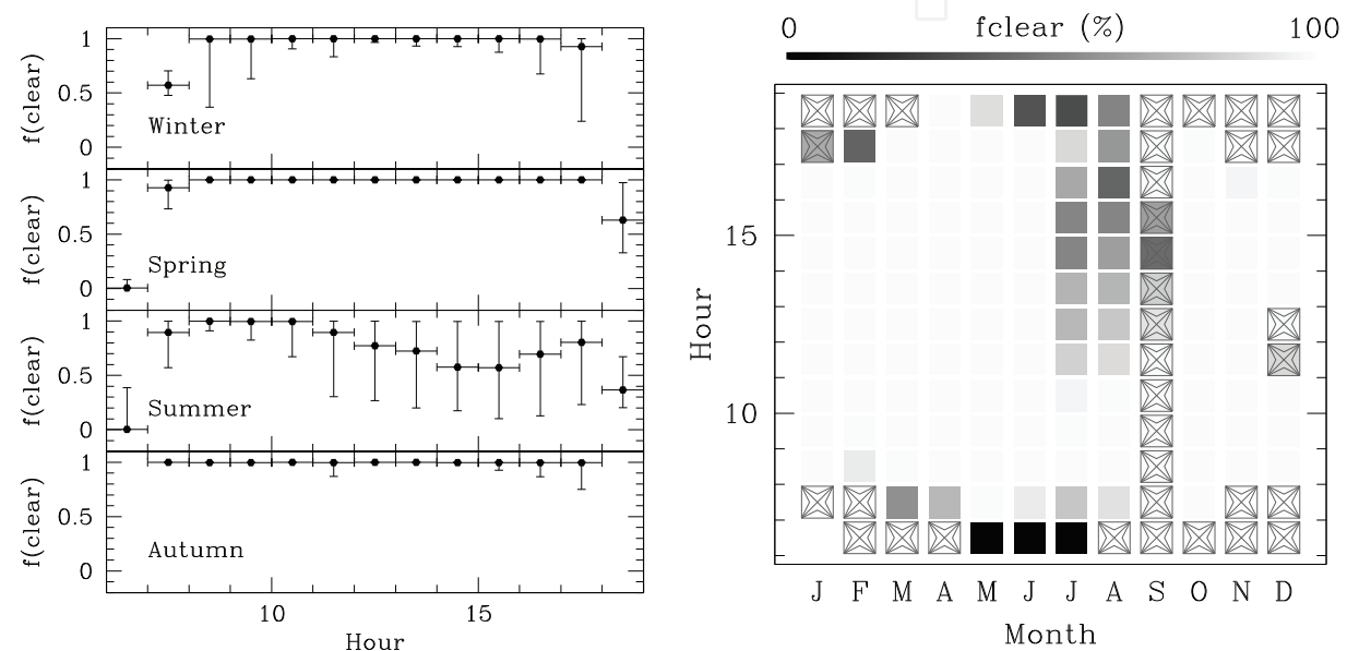
Fig. 18. Left: graph showing the median and quartile values of the fraction of clear weather for each hour of day for each season. Right: a grey level plot showing the median fraction of clear time f(\text{clear}) , for each month and hour of day. Squares are drawn when more than 10 h of data are available; crosses indicate less than 10 h of data.
