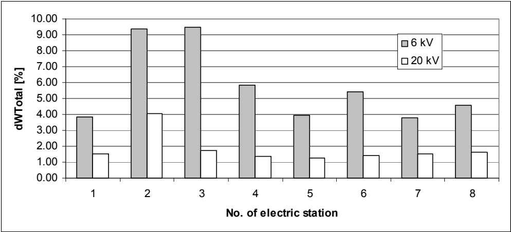
Fig. 14. The annually total energy losses/electric stations
