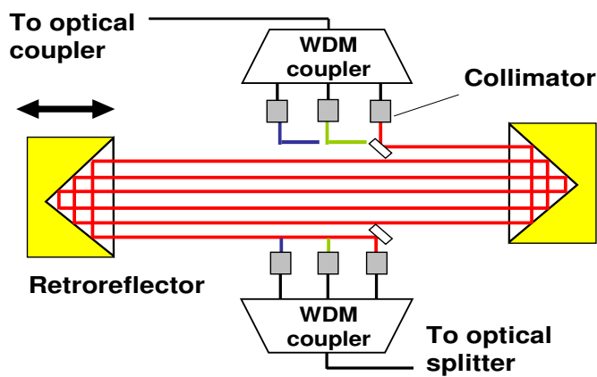
Fig. 8. Free-space optics line length adjuster.
