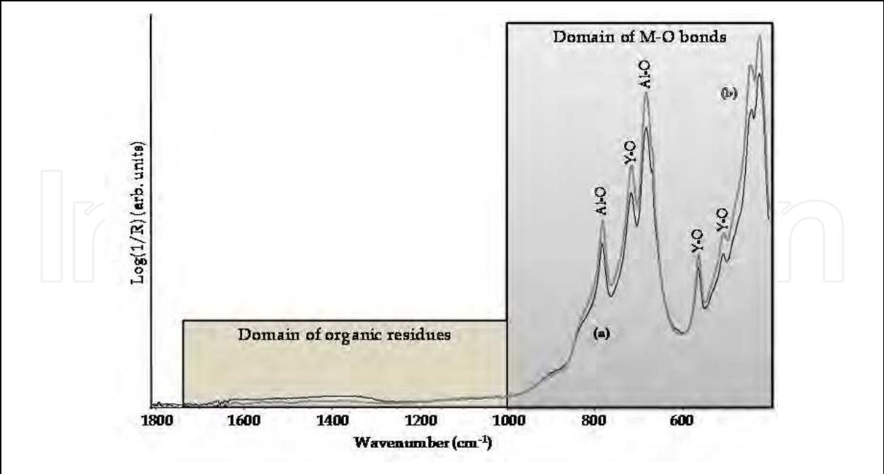
Fig. 9. ATR spectra of YAG:Ce powder synthesized with 3(f/o) th (a) before and (b) after a post-heating treatment at 1000°C for 2 hours.
