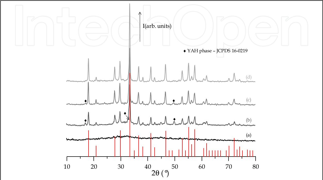
Fig. 5. XRD patterns of undoped YAG powders synthesized with (a) (f/o)_{th} , (b) 2(f/o)_{th} , (c) 2.5(f/o)_{th} and (d) 3(f/o)_{th} , compared to the JCPDS file 33-0040 of YAG.
