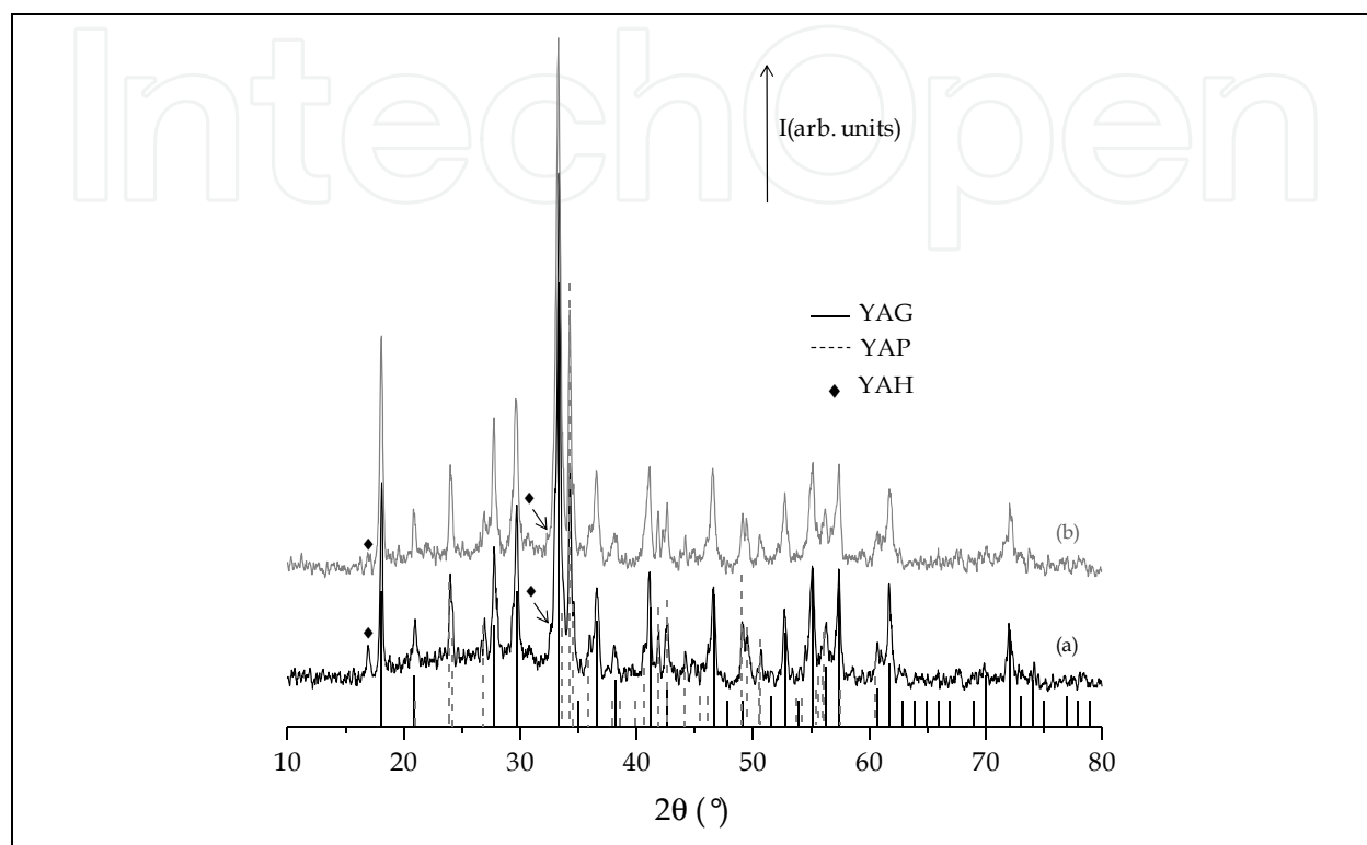
Fig. 8. XRD patterns of YAG:Ce powder synthesized with 3(f/o)_{th} (a) before and (b) after a post-heating treatment at 1000^{\circ}\text{C} for 2 hours, compared to the JCPDS files of YAG (33-0040) and YAP (33-0041).
