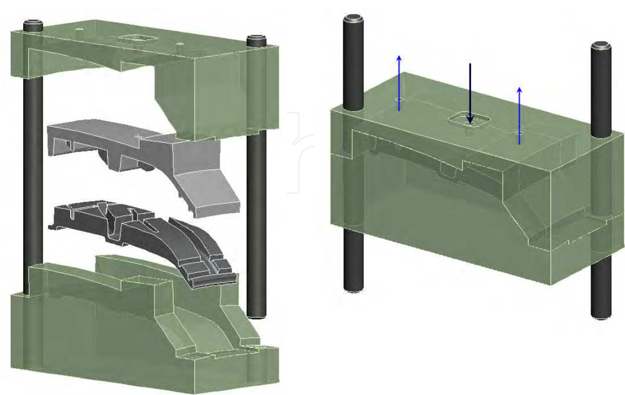
Fig. 11. Die-casting mould.
