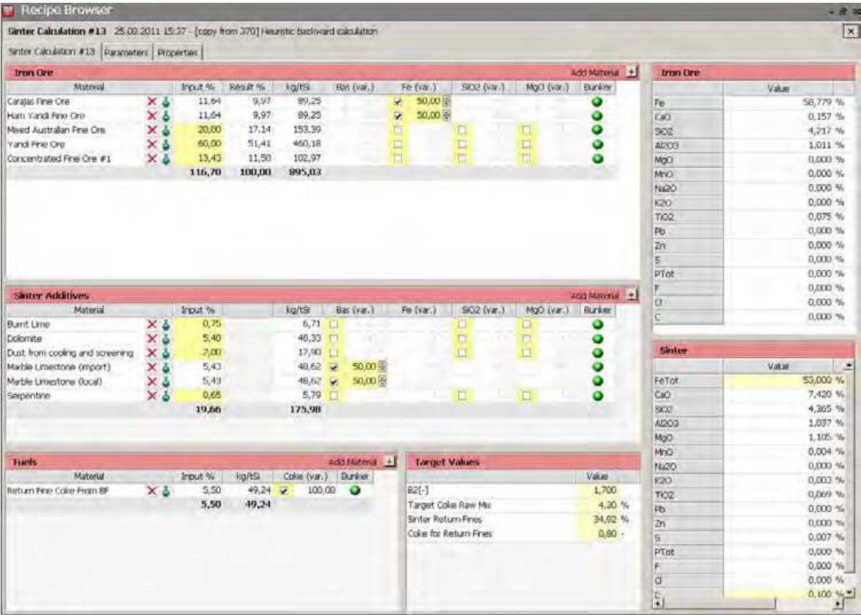
Fig. 4. Raw Mix Calculation for Sinter Plant.
