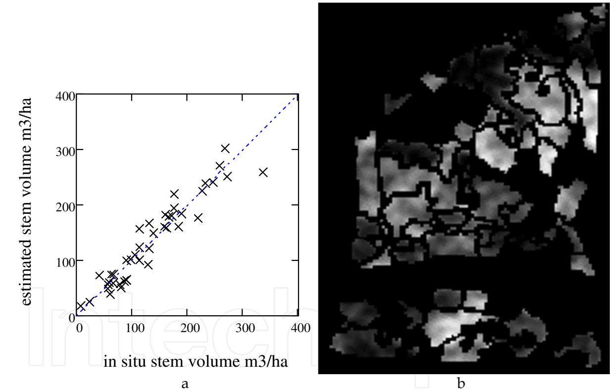
Fig. 11. a: Stand averages of stem volume compared with in situ values; b: Gray scale image of stem volume variation in Kättböle site (stand boundaries marked). The image is normalized such that white corresponds to the highest estimated stem volume of 378 m 3 /ha in a single pixel.
