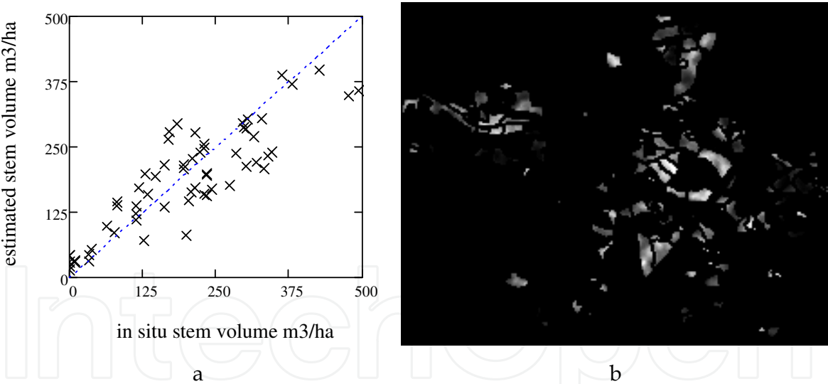
Fig. 15. a: Stand averages of stem volume for 61 stands in Remningstorp compared with in situ values. b: a pixel based map over the Remningstorp stands (white corresponds to maximum estimated stem volume of 491 m 3 /ha).
