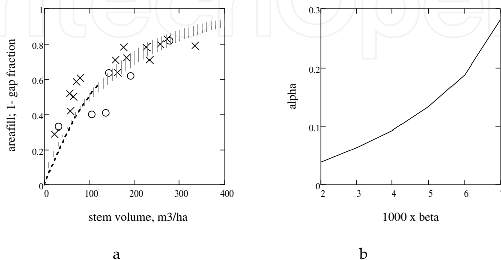
Fig. 1. Observations of areafill/gap fraction, \alpha based on hemispherical photography of Kättböle stands (Santoro et al., 2002), \circ based on results in (Nilson, 1999) from a neighboring area; dashed line: regression line from MODIS observations in Northern Sweden (Västerbotten) (Cartus et al., 2010). Note that the uncertainties in the observations are large. Vertical lines are illustrating range of values of areafill variations for 0.002 < \beta < 0.007 in Eq. (6).
