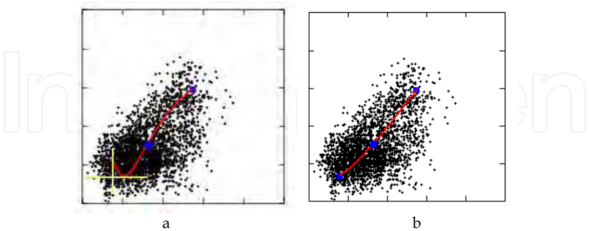
Fig. 14. Illustrating consistency plots for coherence pair 1 and 3, cf Fig. 13, and co-plotted model curve (red lines) for stem volumes from 0 to SVmax. a. IWCM, b. exponential model. The yellow lines, crossing in the point \gamma_{dv} , indicate the levels for the lowest coherence levels for these coherence pairs when the stem volume is \leq SV_{max} . The blue points represent \gamma_{gr} , \gamma_m , and \gamma_{dv} .
