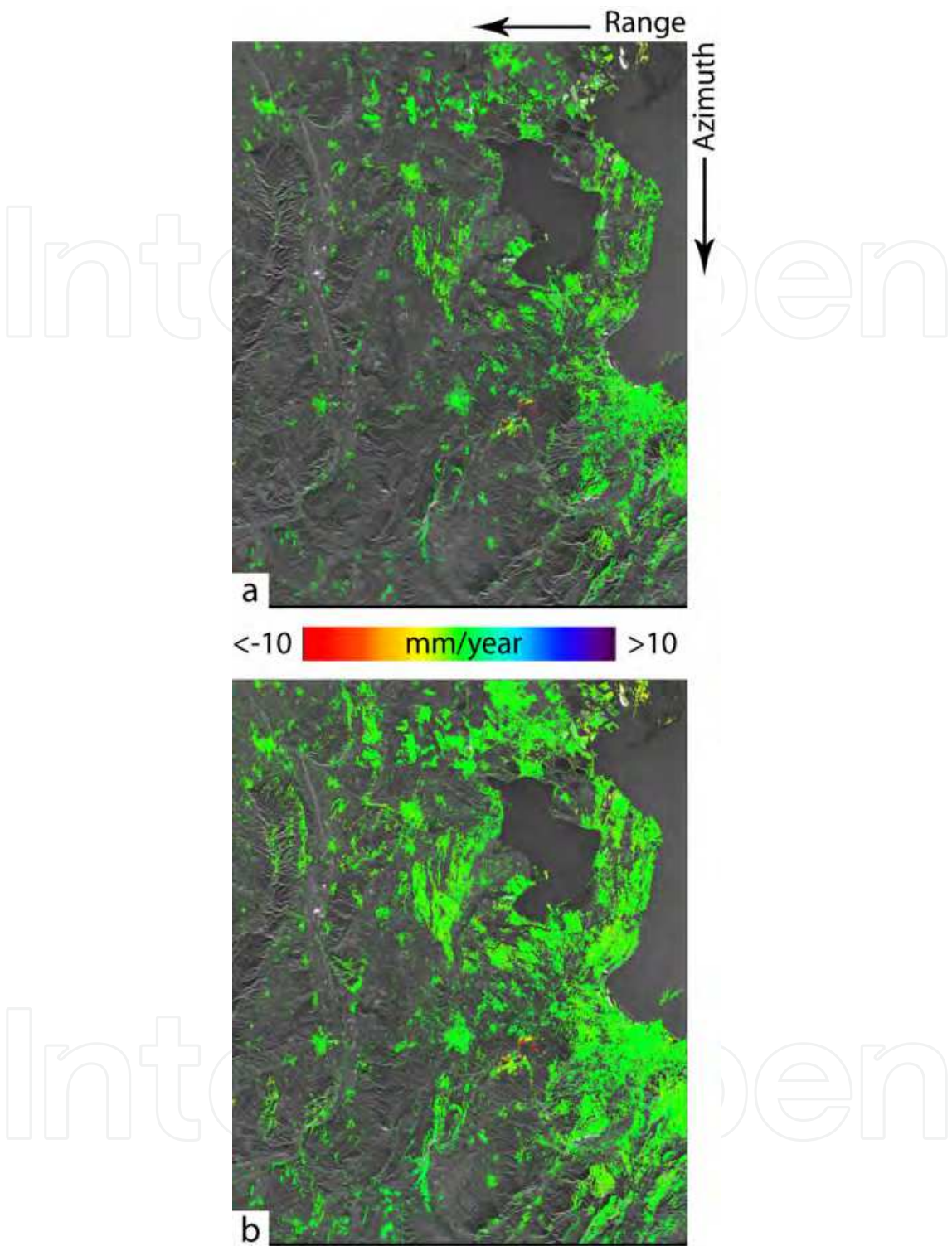
Fig. 9. Mean deformation velocity maps relevant to the Gardanne area (France). a) Conventional SBAS results. b) RG-EMCF results.
