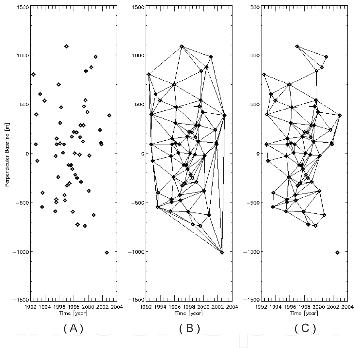
Fig. 3. SAR data representation in the temporal/perpendicular baseline plane for the ERS SAR data analyzed in the following experiments. (A) SAR image distribution. (B) Delaunay triangulation. (C) Triangulation after removal of triangles with sides characterized by spatial and/or temporal baseline values exceeding the selected thresholds (corresponding in our experiments to 300 m and 1500 days, respectively).
