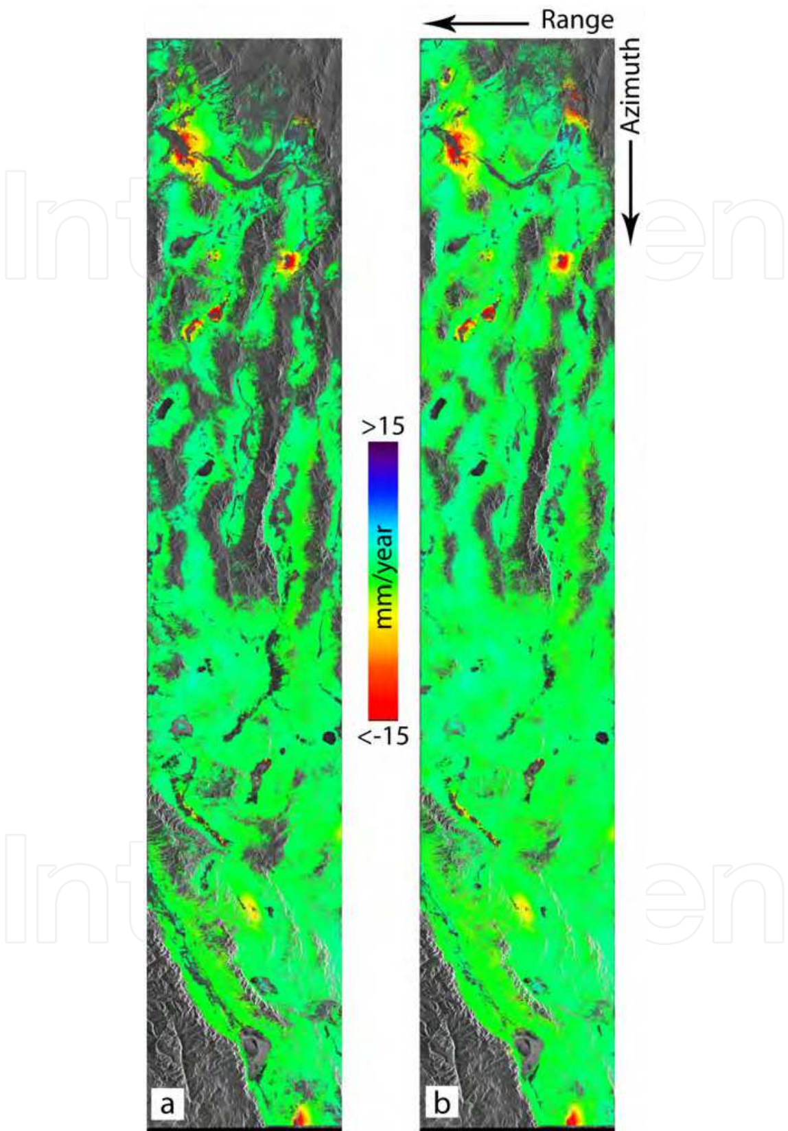
Fig. 7. Mean deformation velocity maps, in SAR coordinates, relevant to Central Nevada area. a) Conventional SBAS results. b) RG-EMCF results. By courtesy of dr. Francesco Casu (Casu, 2009).
