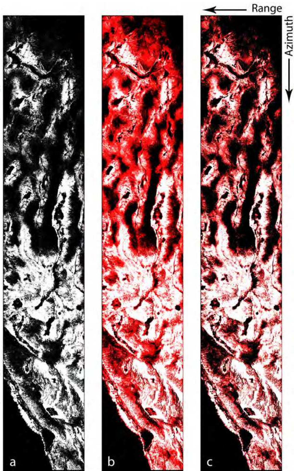
Fig. 6. Temporal coherence masks relevant to Central Nevada area. a) Seed Point mask (~850,000 pixels). b) RG-EMCF results (~1,770,000 pixels). c) Conventional SBAS results (~1,340,000 pixels). Grown points are highlighted in red while in white are represented the Seed Points of Figure 6a. By courtesy of dr. Francesco Casu (Casu, 2009).
