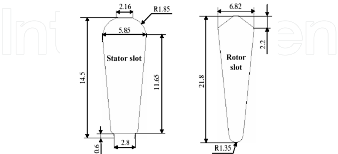
Fig. 7. Gometrical dimensions of the motor slots.
