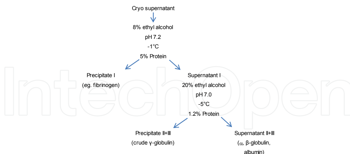
Fig. 1. Cold ethanol fractionation scheme from cryo-supernatant to fraction II+III
