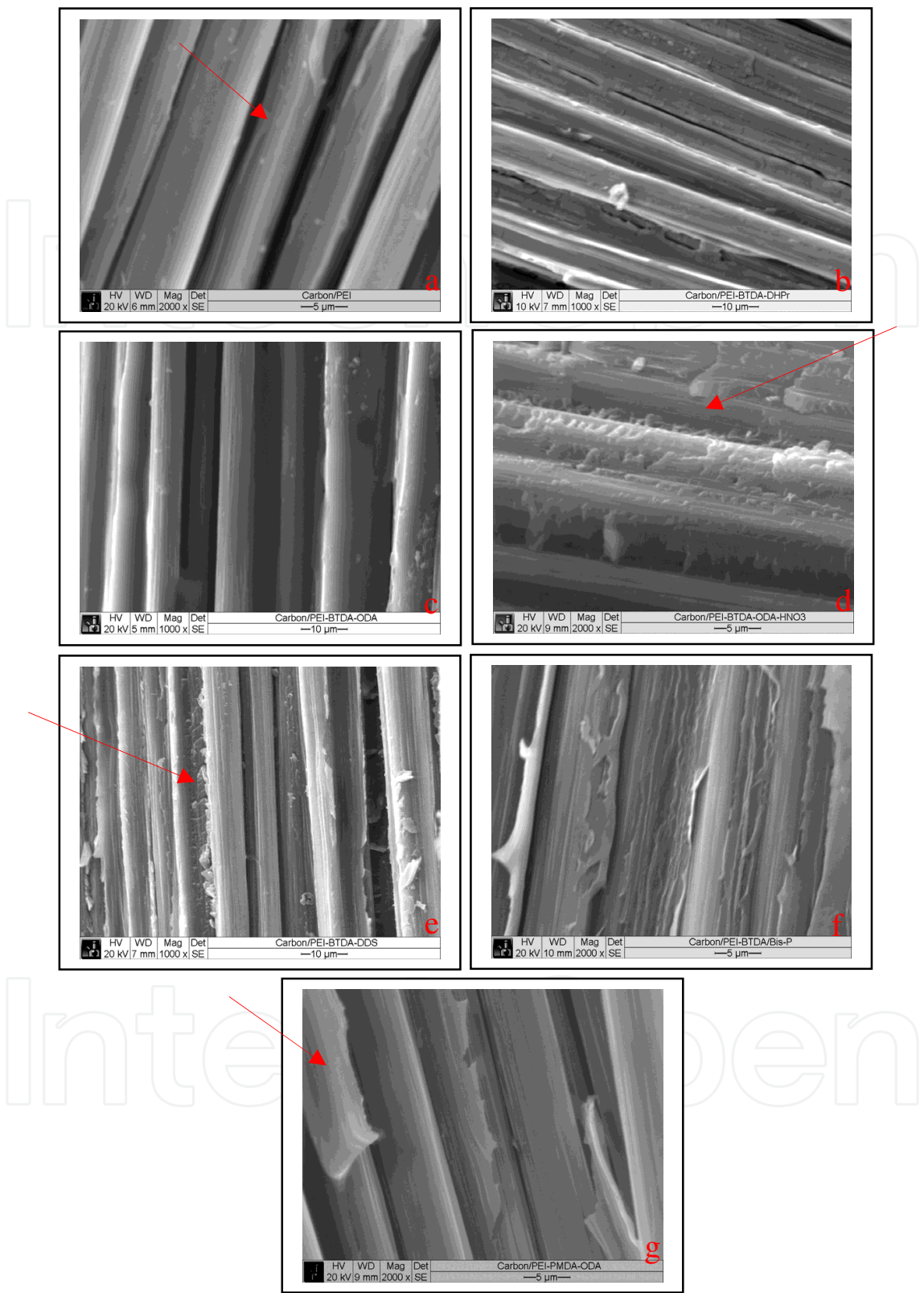
Fig. 8. The fracture surface of the manufactured composites with: a) the hot compression molding and aqueous suspension prepregging b) PI-BTDA/DHPr; c) PI-BTDA/ODA; d) PI-BTDA/ODA-treated fiber with HNO 3 ; e) PI-BTDA/DDS; f) PI-BTDA/BisP and, g) PI-PMDA/ODA.
