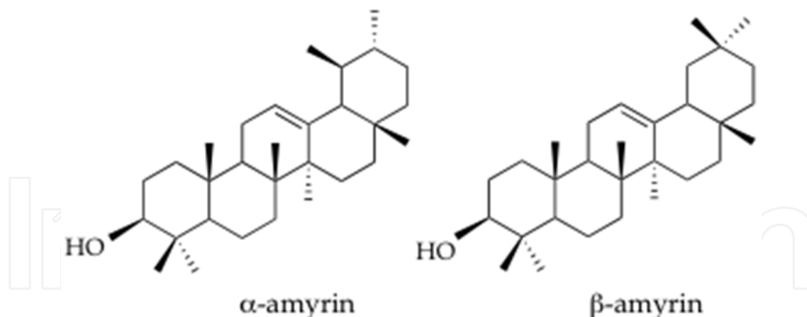
Fig. 1. Estructure of amyrins
