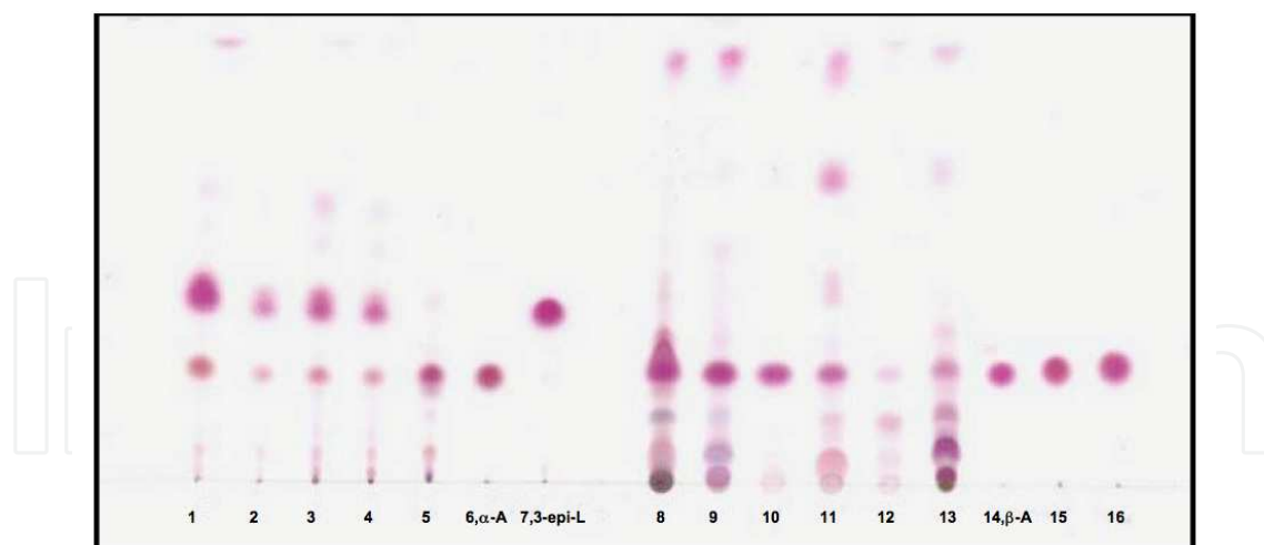
Fig. 2. TLC plate. Tracks: 1=MCT; 2=MCS; 3=MCN; 4=MCP; 5=MER; 6 and 15= \alpha -amyrin; 7=3- epi -lupeol; 8=Dandelion; 9=Olive; 10=Cancerina; 11=Nance wastes; 12=Bearberry; 13=Pot marigold; 14= \beta -amyrin; 15= \alpha -amyrin and 16=mixture \alpha -, \beta -amyrin.
