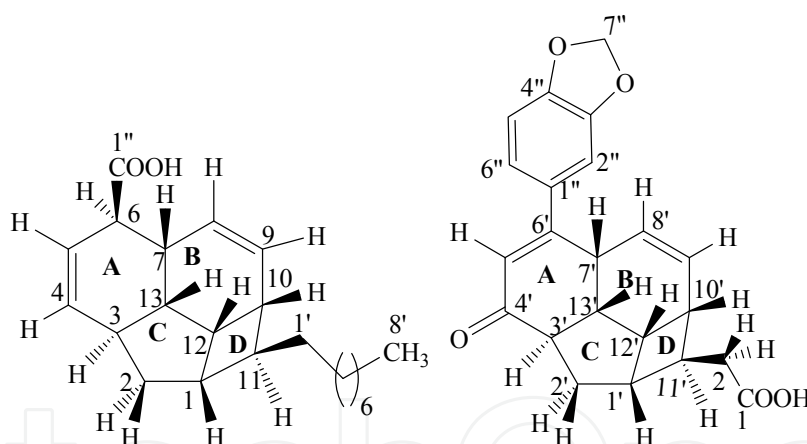
Beilshmiedic acid E ( 5 ) Beilshmiedic acid F ( 6 )
