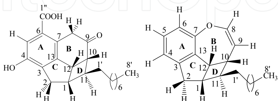
Beilshmiedic acid G ( 7 ) Beilshmiedin ( 8 )
