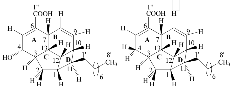
Beilshmiedic acid C ( 3 ) Beilshmiedic acid D ( 4 )
