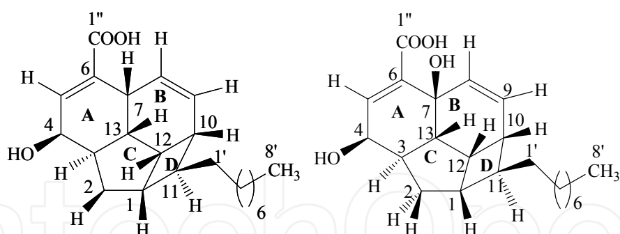
Beilshmiedic acid A ( 1 ) Beilshmiedic acid B ( 2 )
