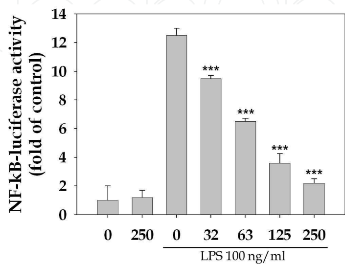
Fig. 5. Effect of EtOAc fraction on LPS-induced NF-κB transcriptional activation. Cells were treated with LPS (100 ng/ml) alone or LPS plus the indicated concentrations (µg/ml) of EtOAc fraction for 24 h. NF-κB activation detected by luciferase reporter assays. *** P < 0.001 vs LPS alone-treated cells.
