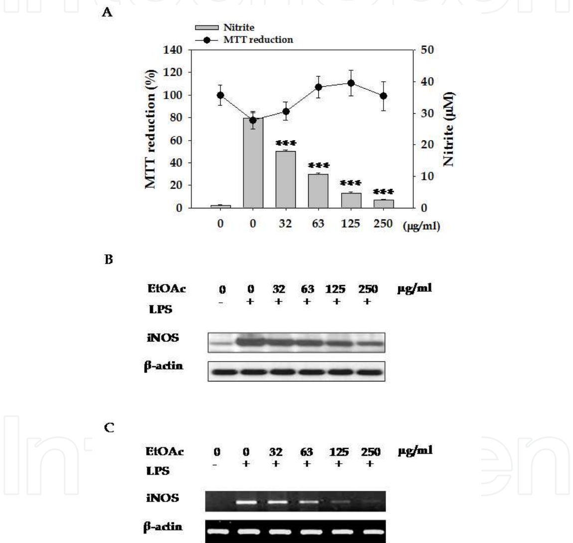
Fig. 1. Effect of EtOAc fraction on the NO production, iNOS protein and iNOS mRNA expression level in LPS-stimulated RAW 264.7 cells. (A) Cells were treated with LPS (100 ng/ml) alone or LPS plus the indicated concentrations of EtOAc fraction for 24 h. *** P < 0.001 vs LPS alone-treated cells. Data are expressed in area density as the mean \pm SD for three independent experiments. (B) Cells were treated with LPS (100 ng/ml) alone or LPS plus the indicated concentrations ( \mu\text{g/ml} ) of EtOAc fraction for 24 h. (C) Cells were co-treated with LPS (100 ng/ml) or LPS with EtOAc fraction at the indicated concentration for 6h. Total RNA was subjected to RT-PCR.
