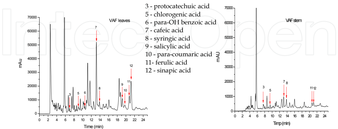
Fig. 4. HPLC chromatograms, used to fingerprint and evaluate quantitatively phenolic acids from leaves and stems of V.album harvested from Fraxinus excelsior (VAF) (Vicas et al., 2011a).
