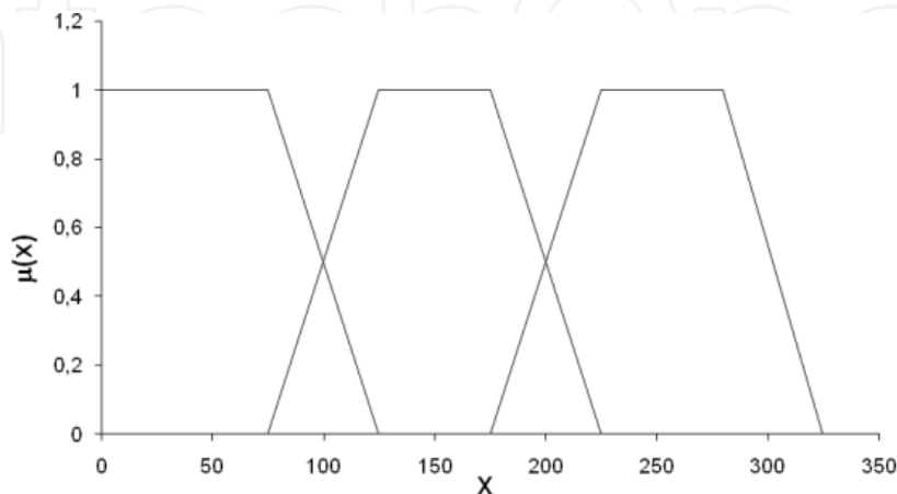
Fig. 2. Membership function.
