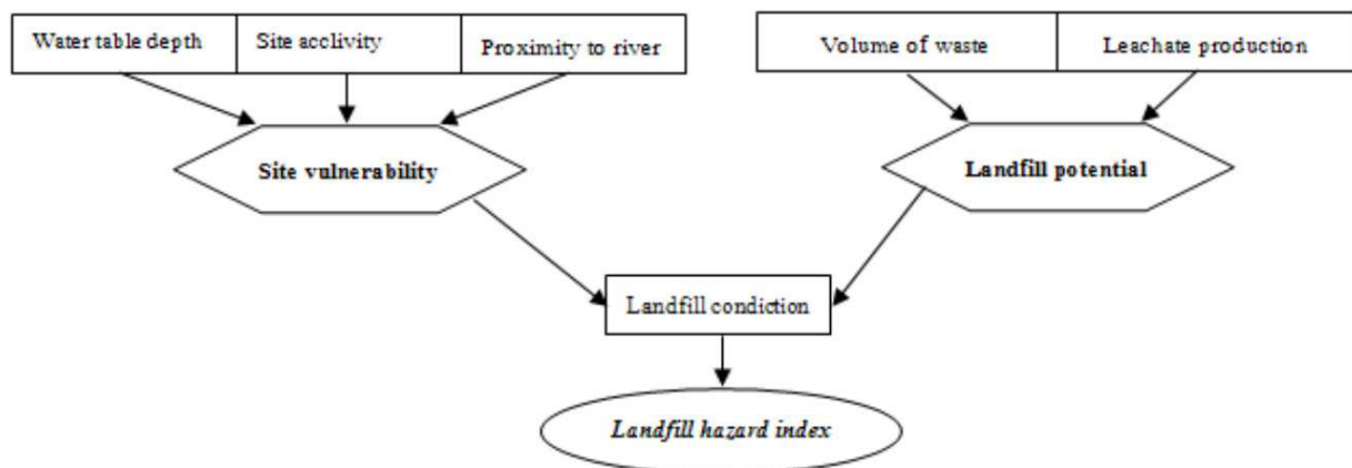
Fig. 17. Conceptual diagram of the implemented fuzzy model.
