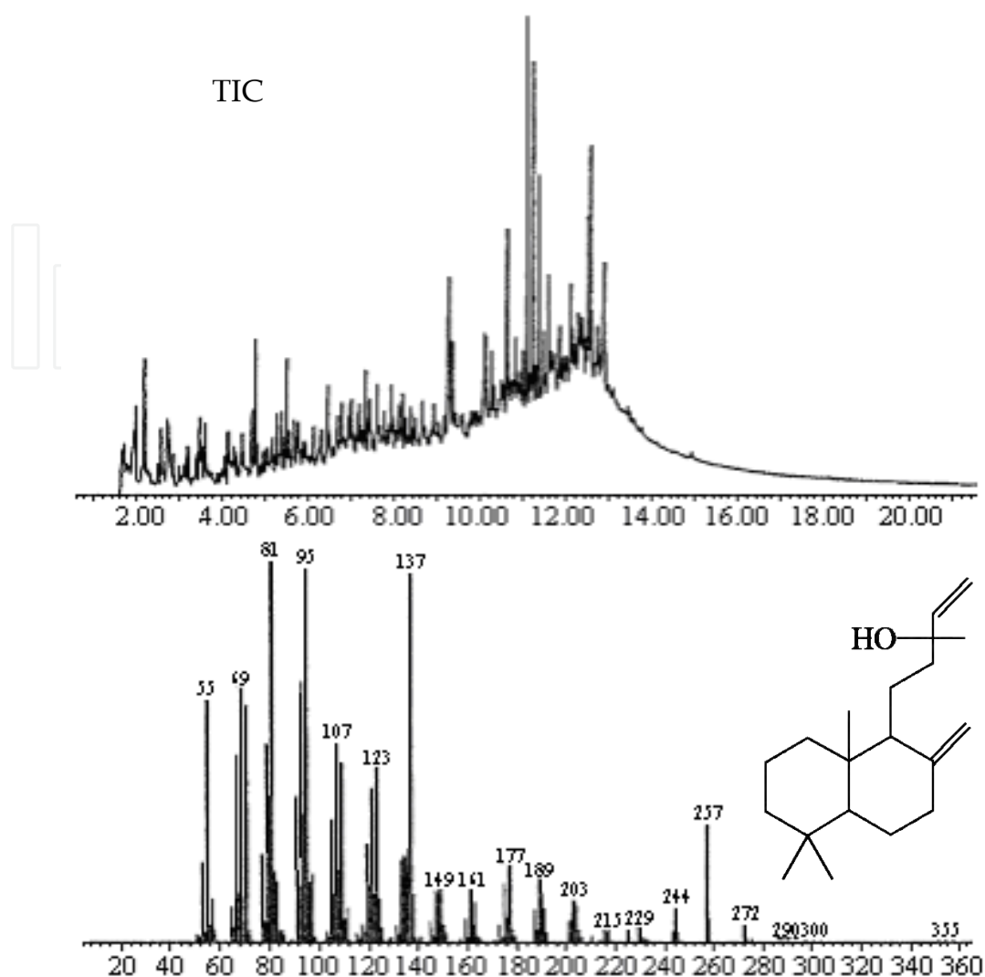
Fig. 4-21. Pyrolysis data of Baroque and Rococo lacquer films
