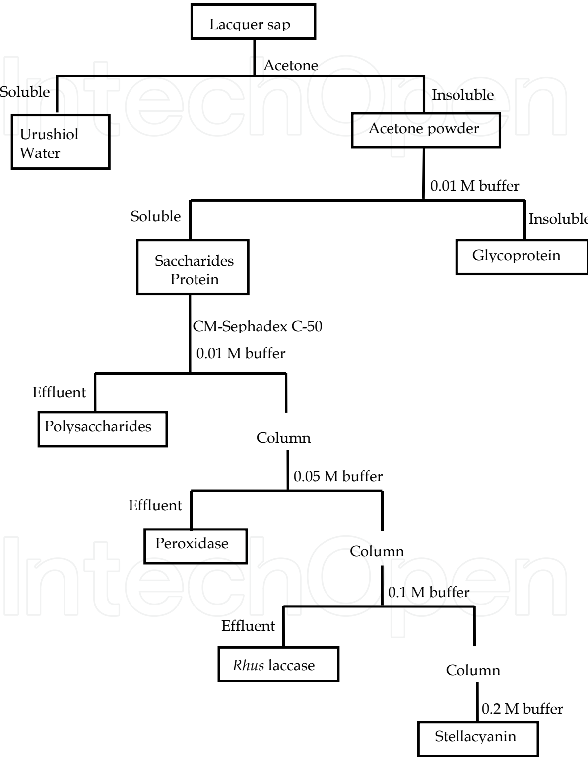
Fig. 1-3. Separation of lacquer sap
