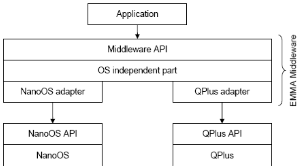
Fig. 10. EMMA Middleware.
