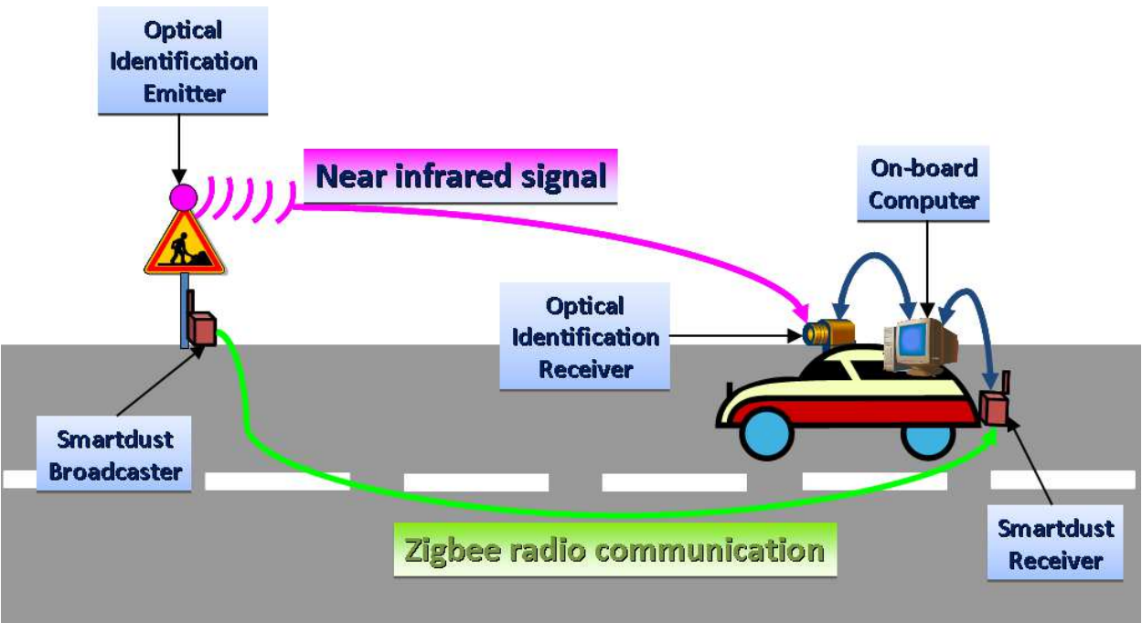
Fig. 7. The set-up of the I2V equipments.
