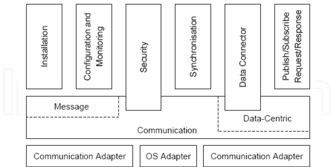
Fig. 11. Modular Components of EMMA Middleware.
