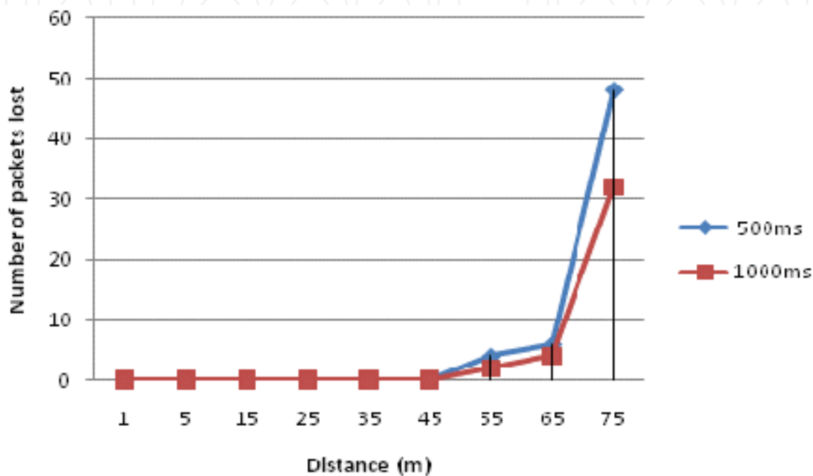
Fig. 15. Urban environment packets lost.
