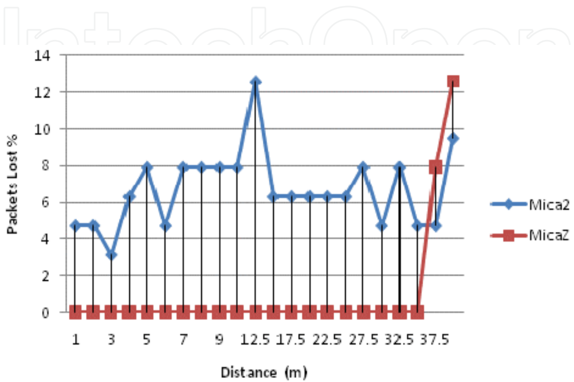
Fig. 4. Packets lost MicaZ vs Mica2.
