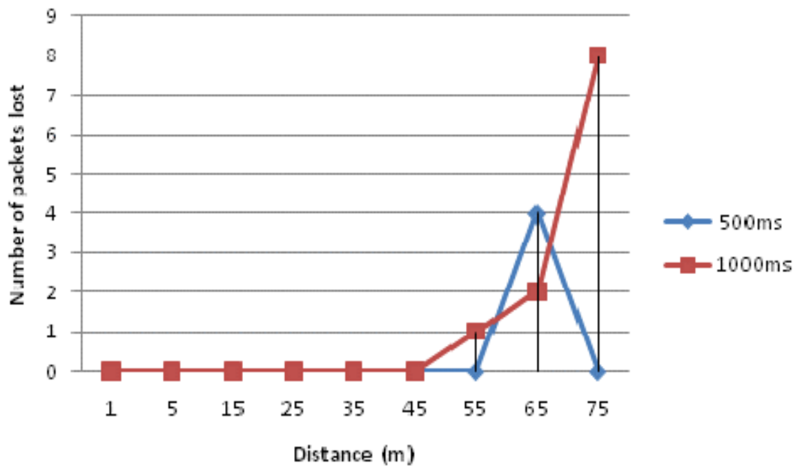
Fig. 14. Open space packets lost.
