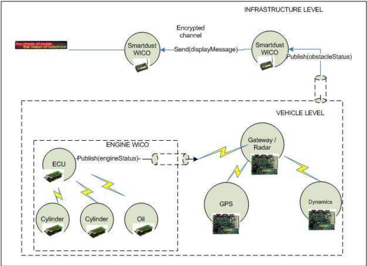
Fig. 13. Inter-hierarchical application.
