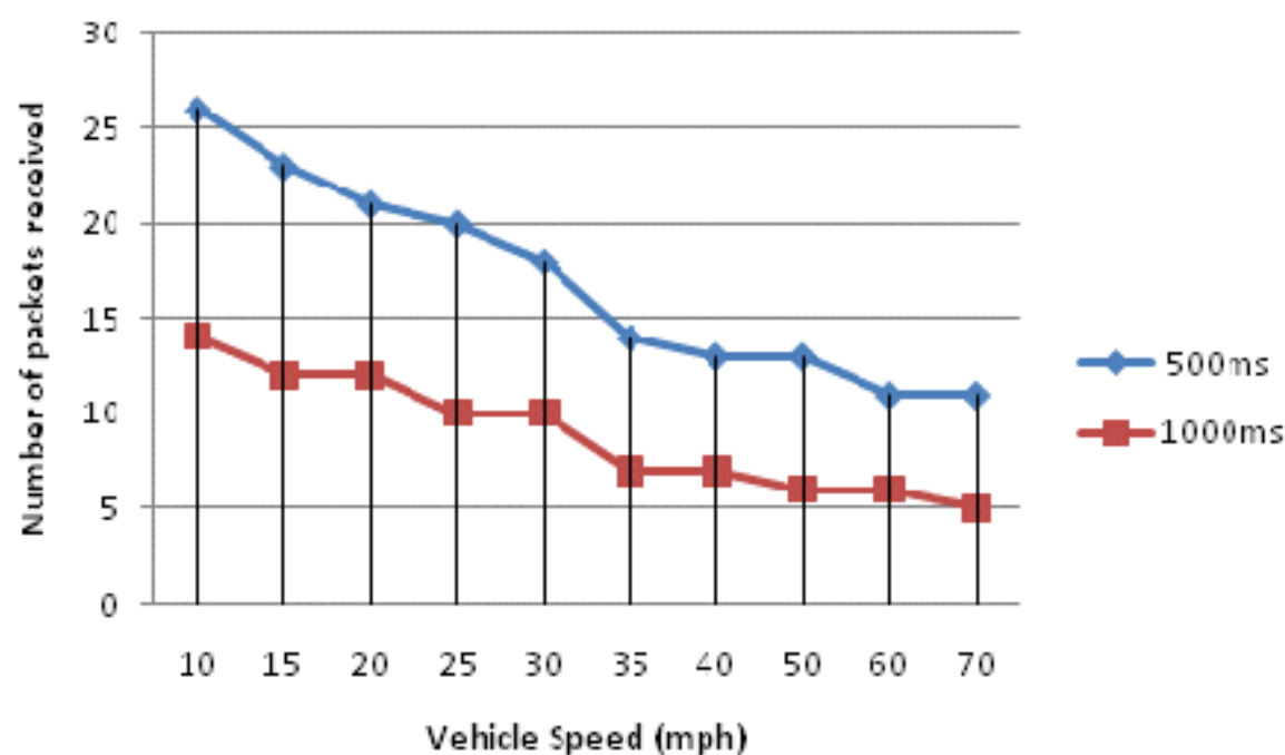
Fig. 16. Mobile environment packets lost.
