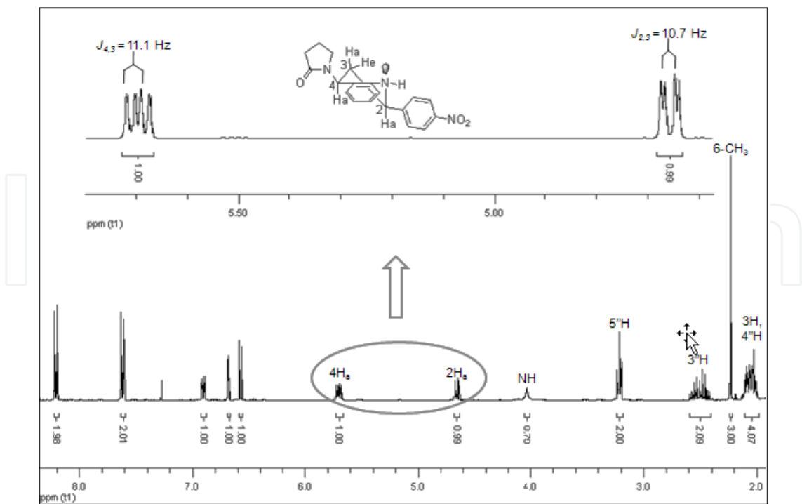
Fig. 6. 1 H NMR spectra of N -[6-methyl-2-(4'-nitrophenyl)-1,2,3,4-tetrahydroquinolin-4-yl]pyrrolidin-2-one 14 .
