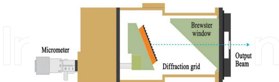
Fig. 1. Schematics of the MTL3-GT TEA laser from Edinburgh Instruments [6]
