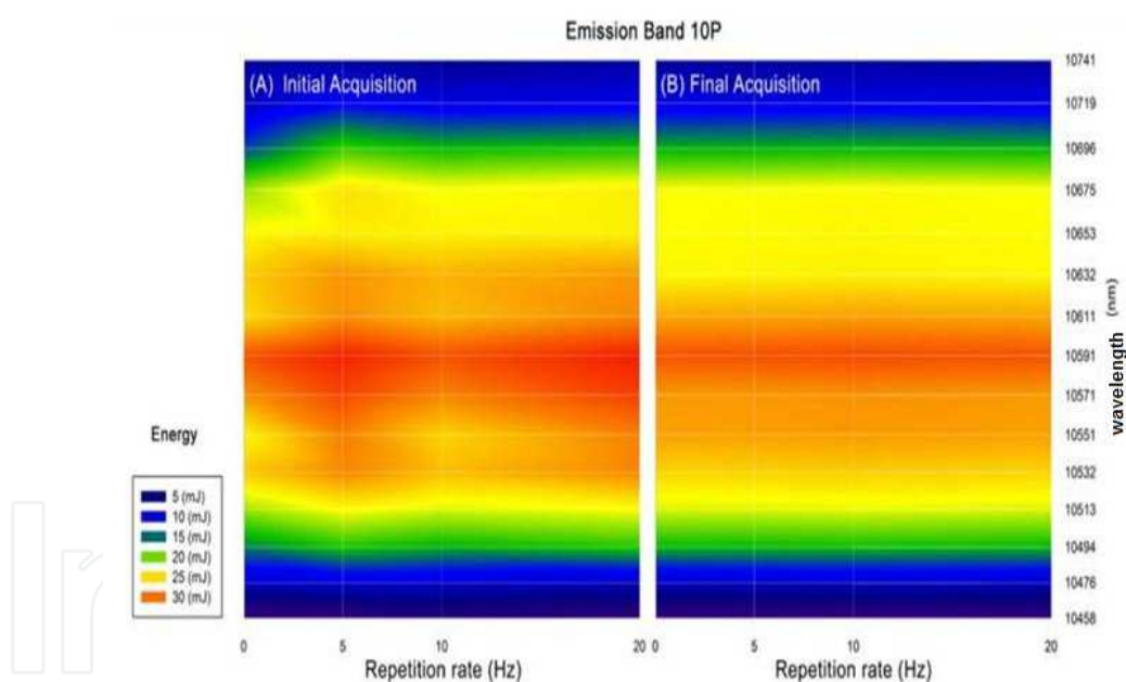
Fig. 2. Relationship between emission line, energy and repetition rates (10P emission band-repetition rates single-shot, 5 Hz, 10 Hz and 20 Hz)
