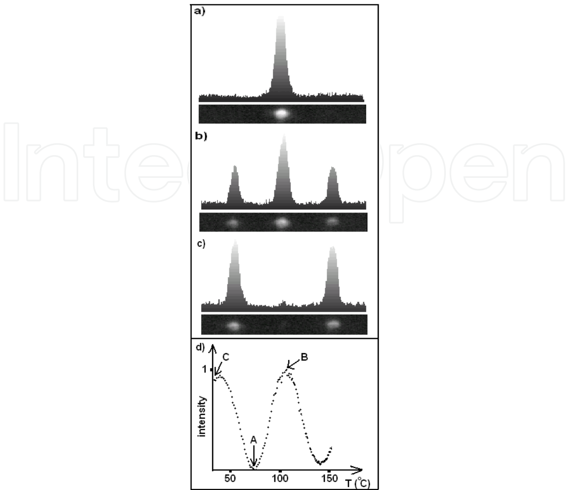
Fig. 15. Diffraction order intensities at different temperatures: (a) T = 77\text{ }^{\circ}\text{C} , (b) T = 108\text{ }^{\circ}\text{C} , and (c) T = 140\text{ }^{\circ}\text{C} . The maximum intensity is normalized to unity. (d) Experimental result of the intensity of the 1st order of diffraction versus temperature. The maximum intensity is normalized to unity (Riahi et al, 2008).
