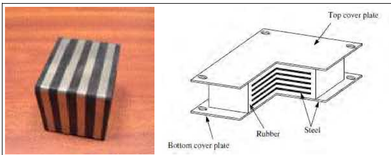
Fig. 5. Seismic isolator, laminated rubber bearing (LRB).
