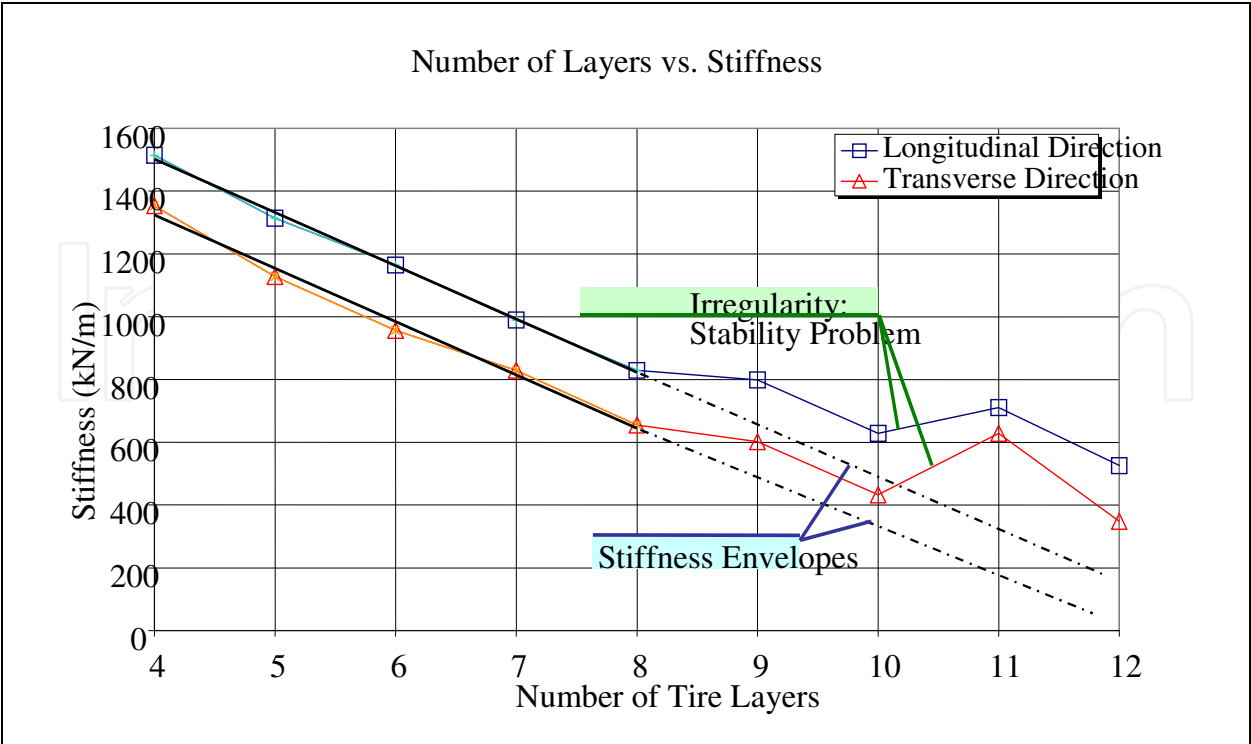
Fig. 7. Stability graph of scrap tire pads (STP).
