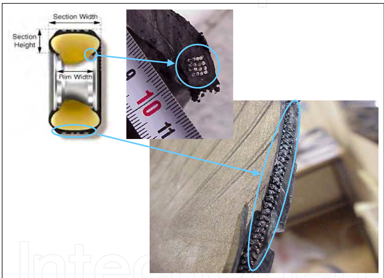
Fig. 9. Typical cross section of a scrap tire.
