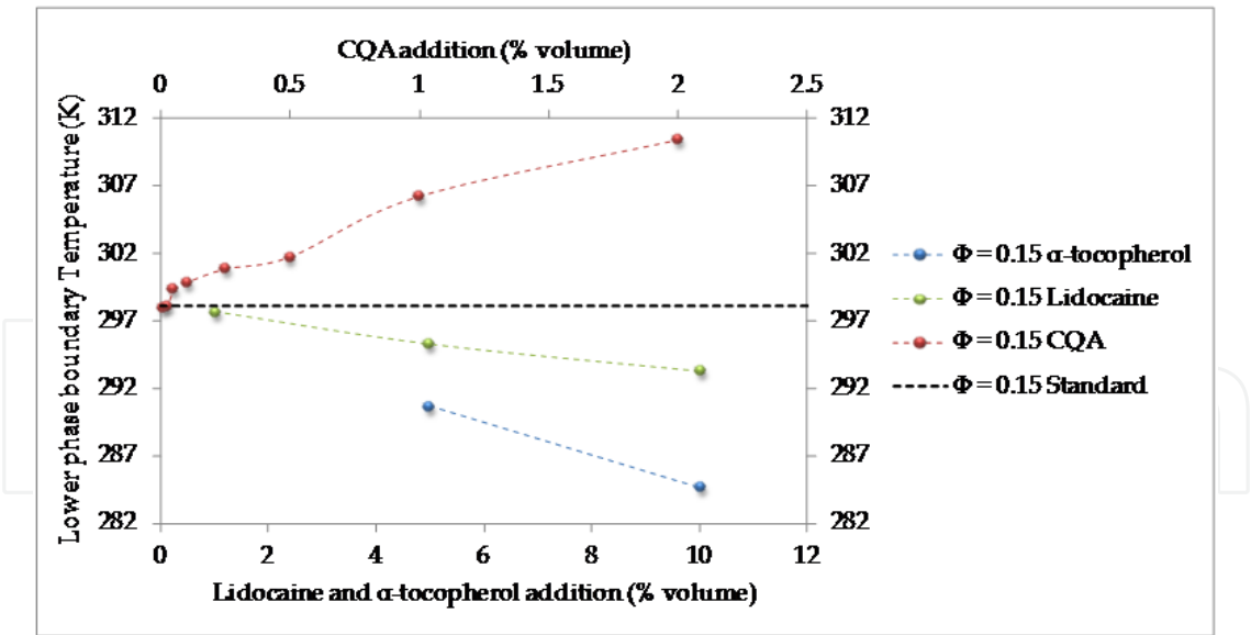
Fig. 9. Partial phase diagram in the water rich region with the surfactant and oil concentrations fixed at \Phi = 0.15 with varied amount of the oil substituted with \alpha -tocopherol and lidocaine, and water substituted with CQA.
