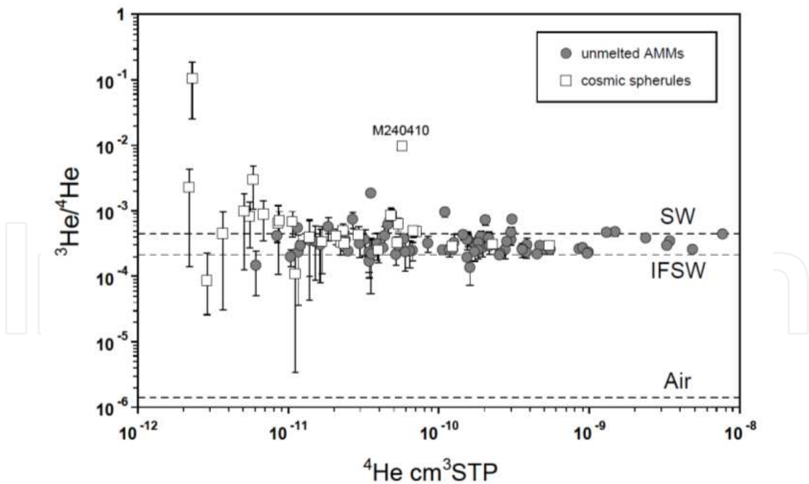
Fig. 4. Relationship between ^4\text{He} content and ^3\text{He}/^4\text{He} ratio of unmelted AMMs and cosmic spherules. Unmelted AMM data are from Stuart et al. (1999), Osawa and Nagao (2002b), and Osawa et al. (2003). Cosmic spherule data are from Osawa and Nagao (2003) and Osawa et al. (2010).
