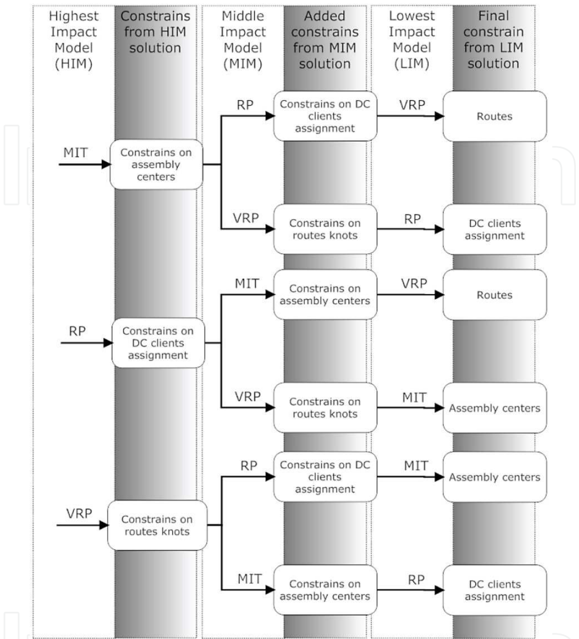
Fig. 10. Possible combinations of priorities
