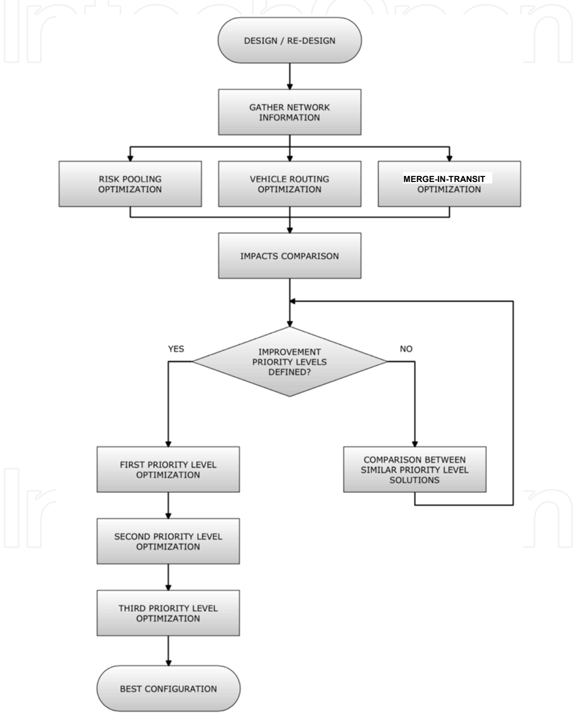
Fig. 9. Applied framework
