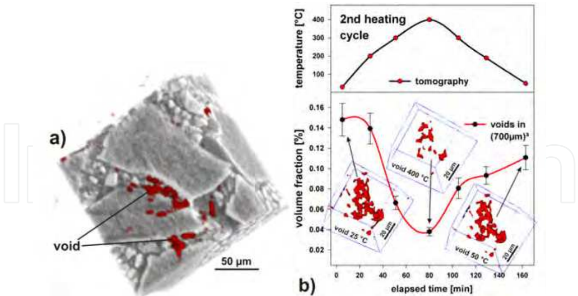
Fig. 13. Voids in an AlSi7Mg/SiC/70p composite during thermal cycling (RT – 400 °C). a) A single void between large SiC particles compared to b) evolution of the void volume fraction during thermal cycling (Schöbel et al. 2011).
