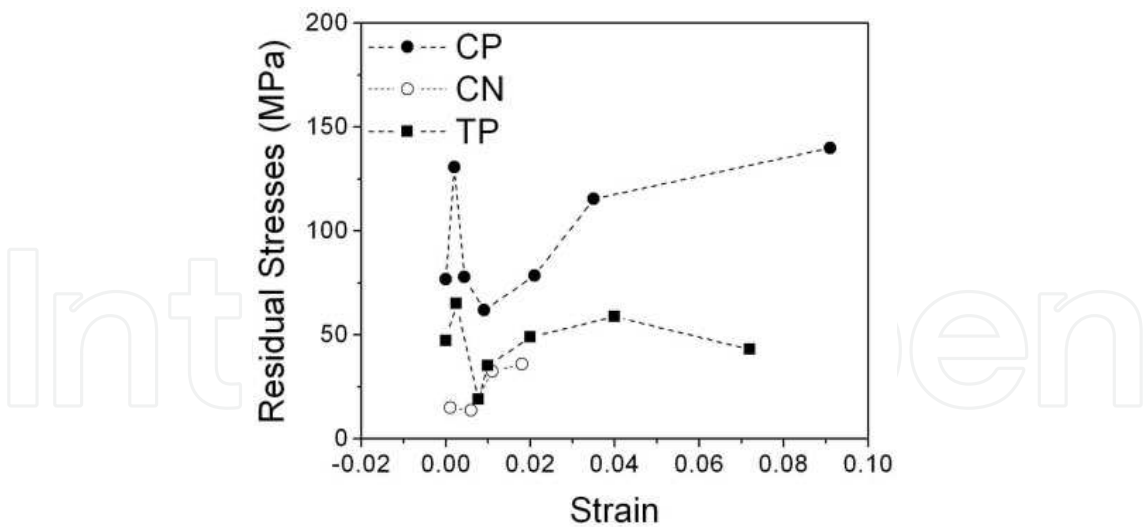
Fig. 18. Von Mises stress in an Al/ Al 2 O 3 /15s SFRM as a function of pre-strain accumulated in the composite for the three loading modes: CP (compression in plane), CN (compression out of plane) and TP (tension in plane) (Garcés et al., 2006b).
