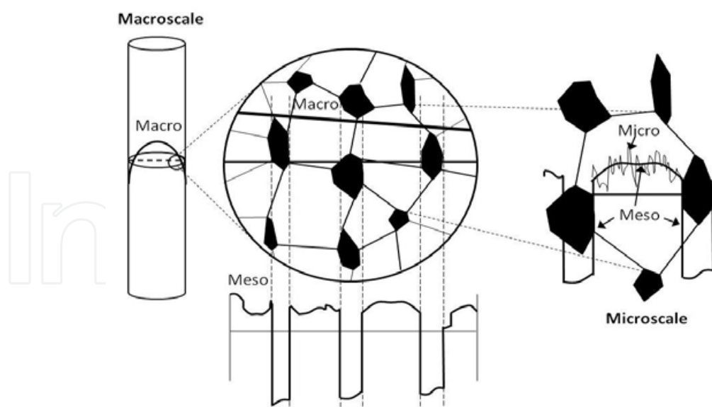
Fig. 3. Schematic view of the residual stresses that can arise in the different structural scales of a PRM. Ceramic particles are indicated as black regions.
