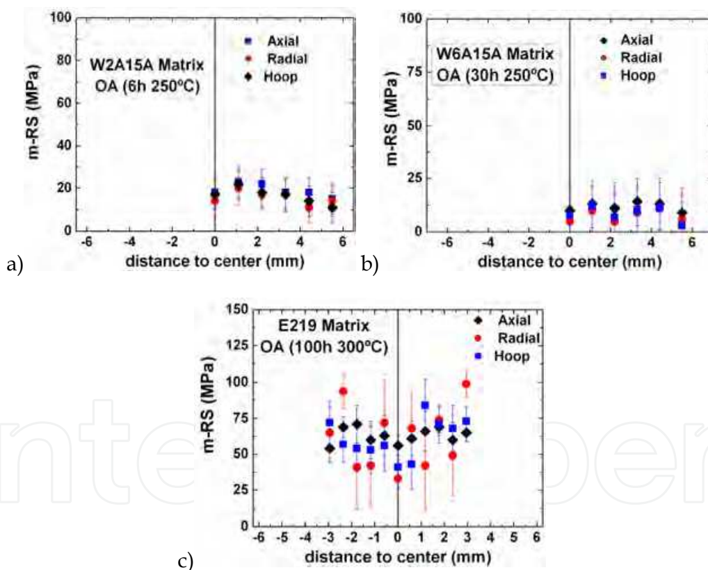
Fig. 10. Relaxation of microstresses after thermal treatment for: a) IM 2014/ \text{Al}_2\text{O}_3 /15p, b) IM 6061/ \text{Al}_2\text{O}_3 /15p, c) PM 6061/SiC/15w (Fernández et al., 2011).
