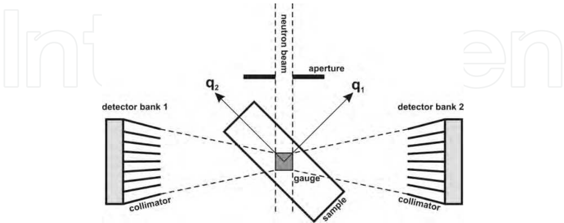
Fig. 6. TOF setup with two detector banks at fixed \theta positions.
