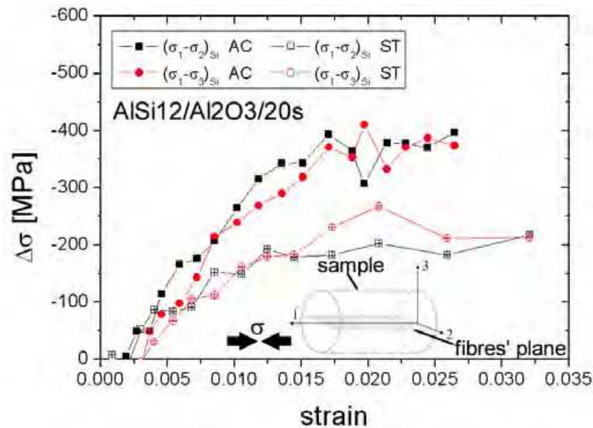
Fig. 21. Evolution of the stress differences ( \sigma_1-\sigma_3 ) and ( \sigma_1-\sigma_2 ) in AlSi12/Al 2 O 3 /20s determined by in situ neutron diffraction for the eutectic Si in the AC and 540°C/4h conditions as a function of the applied compressive strain. The geometry of the sample and the orientation of the fibres' plane (1-2) with respect to the applied stress \sigma (1) are indicated (Requena et al. 2009a).
