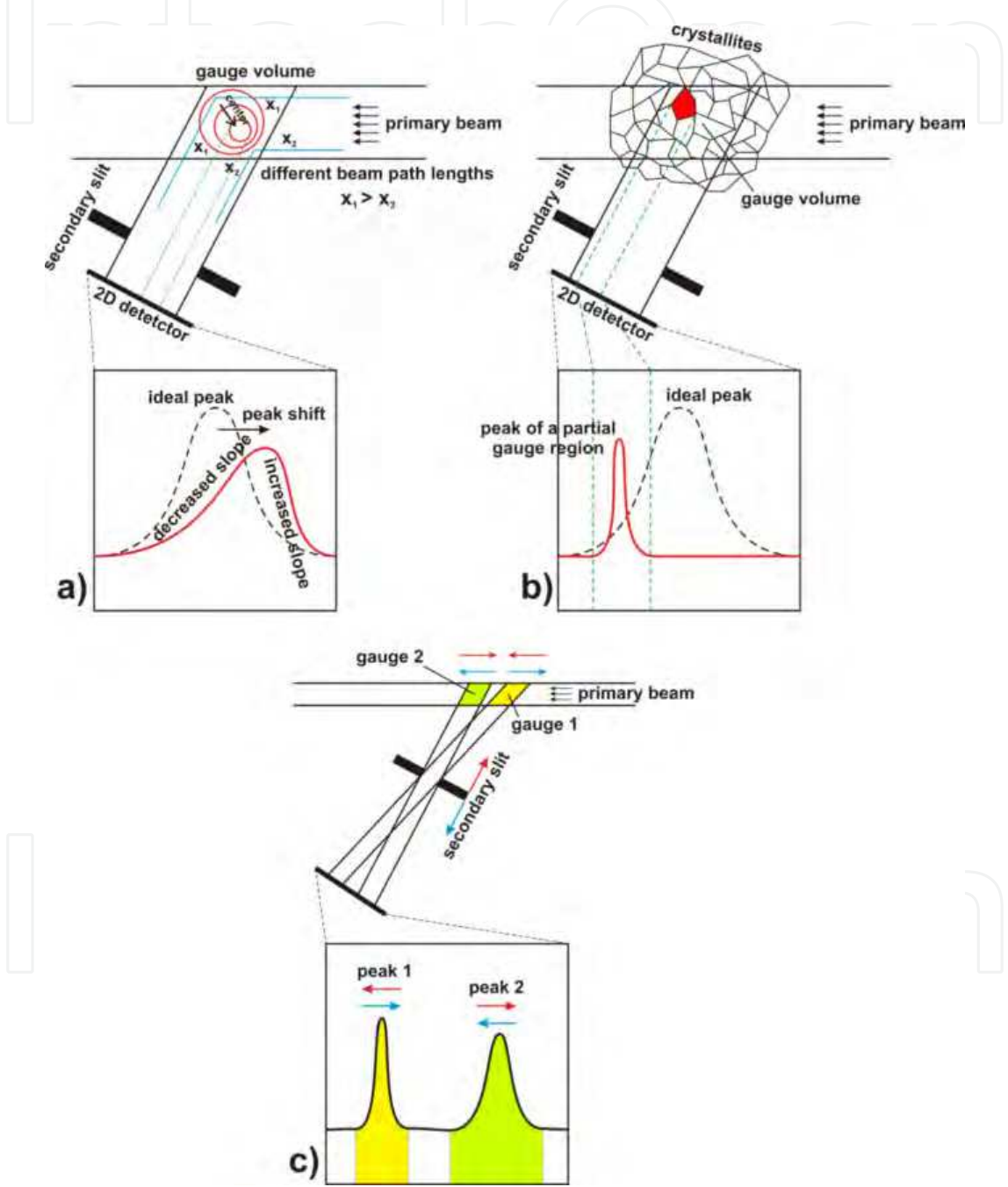
Fig. 7. Systematic errors that can occur using an angle dispersive diffraction setup (Schöbel, 2011a): a) displacement of the diffraction centre from the centre of the gauge volume due to absorption effects, b) coarse grains and c) pseudo micro strains generated by a change of the secondary-slit-to-sample distance.
