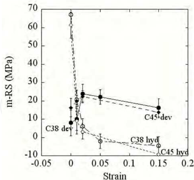
Fig. 17. Hydrostatic (hyd) and deviatoric (dev) microstress evolution in the aluminium phase with plastic deformation for two PM 6061/SiC/15w MMC (C38, C45) (R. Fernández et al., 2005).
