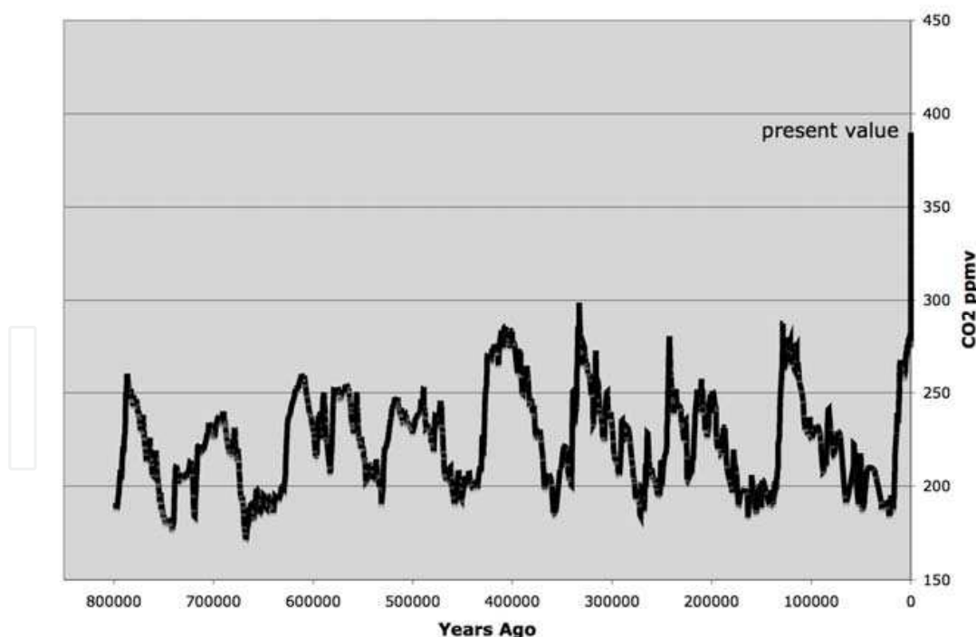
Fig. 1. Record of atmospheric CO 2 in ppmv 800,000 years ago to the present. Ice core data from Supplementary materials in Luthi et al, 2008, including Monnin et al, 2001; Pepin et al, 2001; Petit et al, 1999; Raynaud et al, 2005; Siegenthaler et al, 2005. Data from 1958 CE onwards, Keeling et al, 2001, and Keeling et al, 2011
