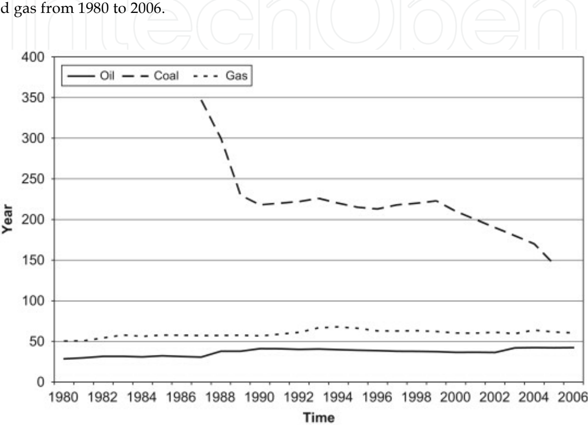
Fig. 4. The ratios of world consumption to reserves for oil, coal and gas from 1980 to 2006.
