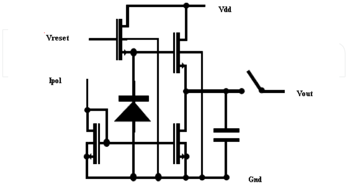
Fig. 12. Schematic structure of the CMOS sensor proposed for charged particle detection.
