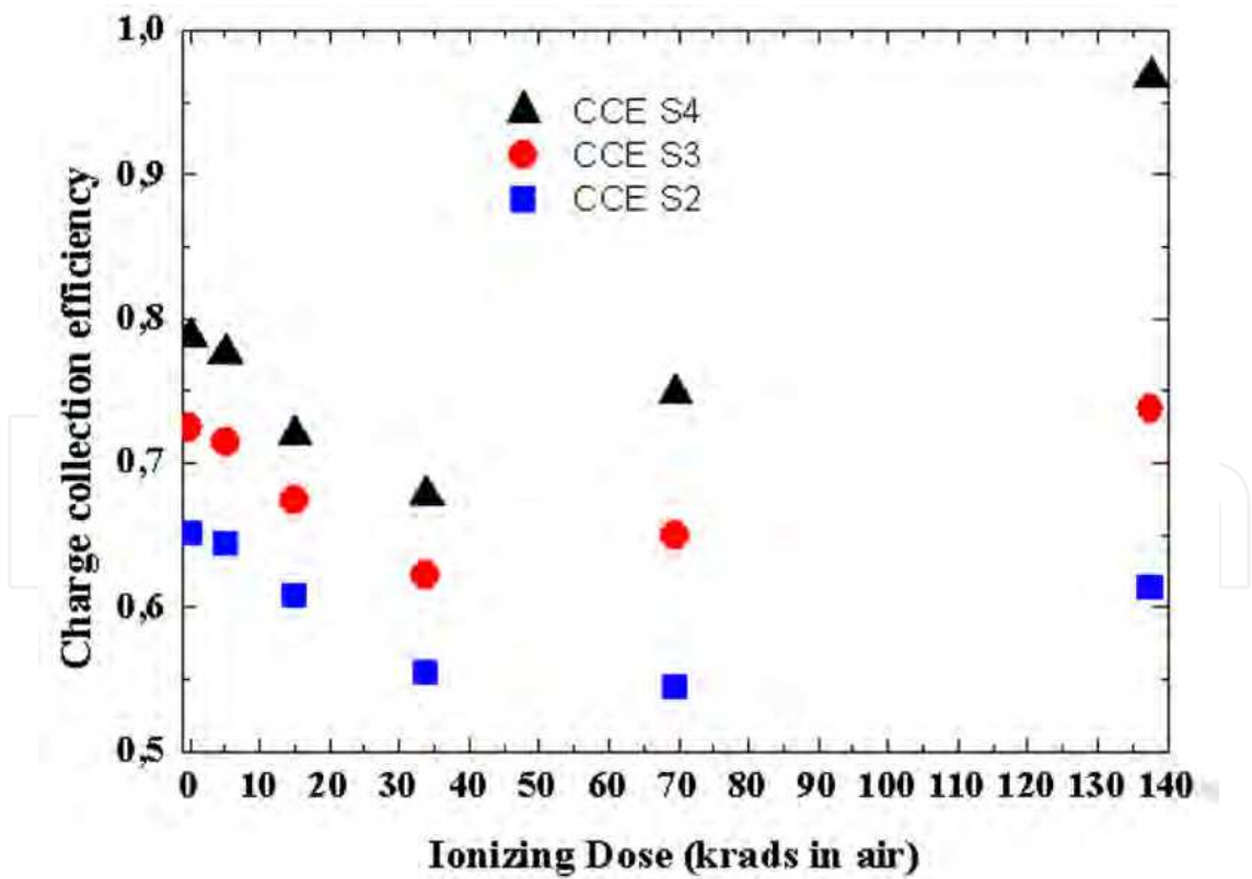
Fig. 13. CCE versus TID for different sensor diode sizes: (S4, S3, S2). The increase in the CCE along with the TID could find its origin in a high surface local electric field, which results in carrier multiplication.
