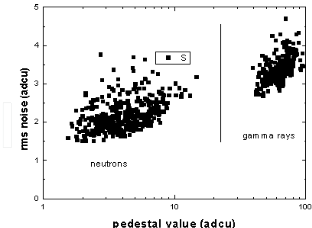
Fig. 14. Root Mean Square value of the temporal noise plotted versus the corresponding Pedestal (offset) values for pixels irradiated with neutrons (left) and pixels irradiated at a dose of 137 krad (Si)(right).
