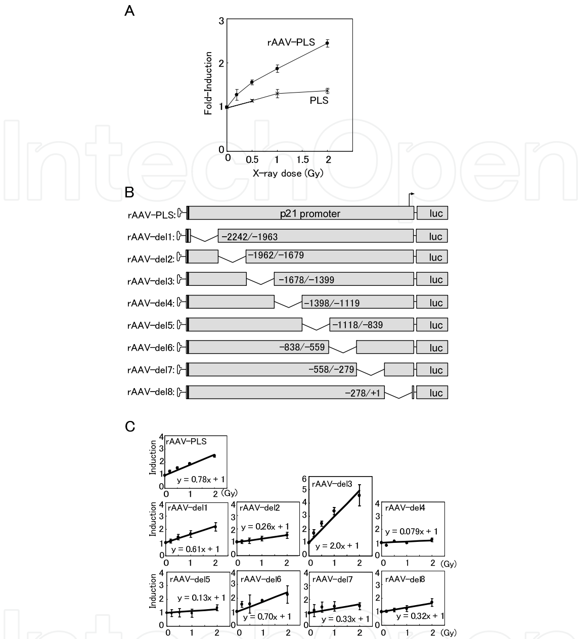
Fig. 12. DNA regions functioning in the IR response of the CDKN1A gene. A: Reporter gene constructs containing the luciferase gene under the control of the CDKN1A gene promoter were either transfected by electroporation (PLS) or transduced by rAAV vectors (rAAV-PLS) into MCF-7 cells. The cells were irradiated with X-rays and assayed for luciferase activity 5 h after irradiation or mock treatment. Results are the means of three independent experiments. Error bars represent the S.D. B: The reporter gene constructs with or without deletions in the 5' flanking region are schematically represented. The TP53 site at -2.2 kb is indicated by a heavy line. These constructs were transduced into MCF-7 cells using rAAV vectors. C: X-ray response of each construct was assayed in the dose range of 0.2-2.0 Gy. Since the fold induction increased linearly with dose, the slope was used as an index of IR responsiveness. Results are the mean of three independent experiments. Error bars represent the S.D. (Reproduced with permission of Elsevier B. V. from Ref (Nenoi et al., 2009))
