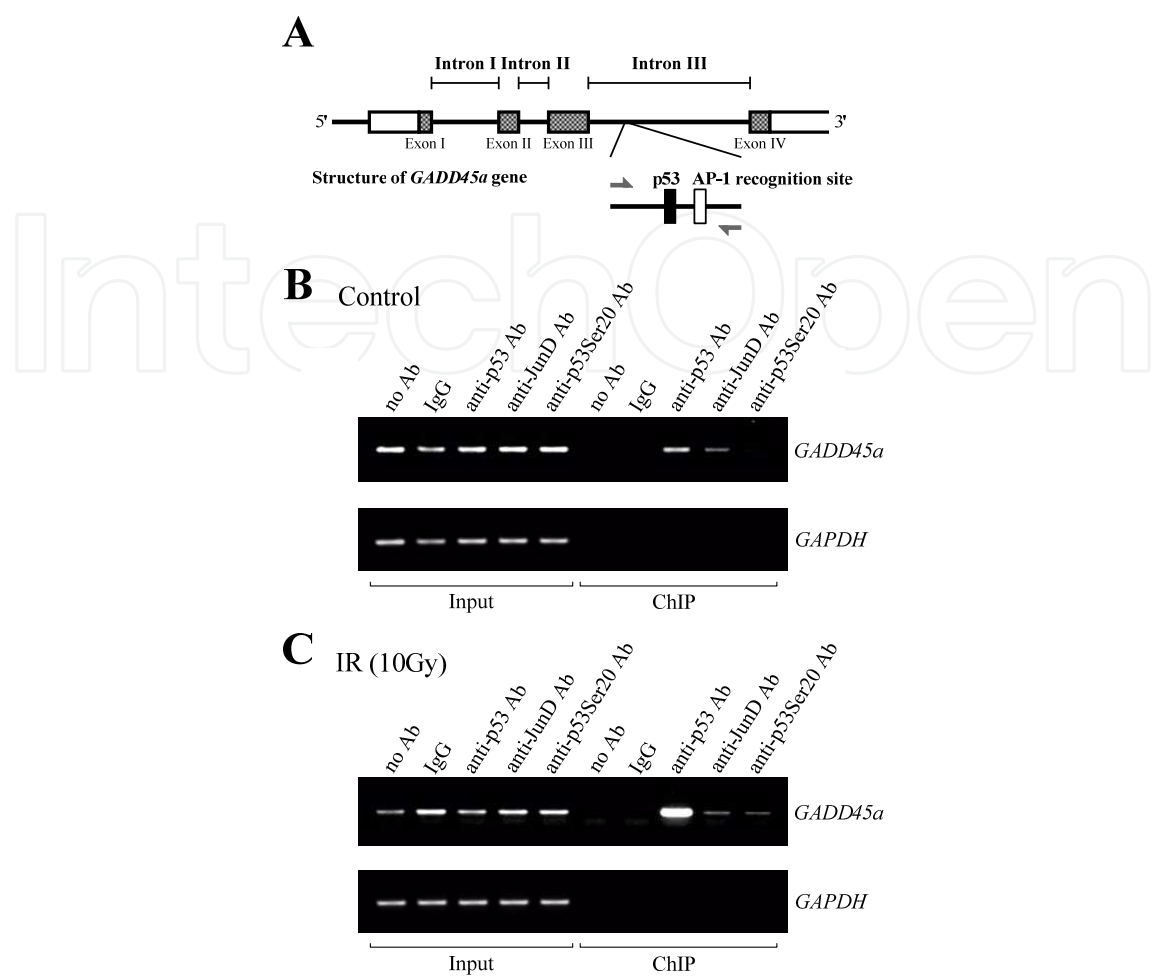
Fig. 10. Chromatin immunoprecipitation (ChIP) analysis for the in vivo binding of JunD at the third intron. (A) Schematic illustration of genomic structure of the GADD45A gene. PCR primers were designed to amplify the region containing both the p53 site and the AP-1 site, as represented by arrows. (B) ChIP analysis was performed with MCF-7 cells, unirradiated (B) or exposed to 10 Gy of X-rays with 1.5 h postincubated (C). Sheared chromatin was incubated without antibodies (no Ab) or with the IgG, anti-p53 antibody, anti-JunD antibody, and anti-phospho-p53 (Ser20) antibody. Immunoprecipitants were analyzed by PCR. The GAPDH promoter containing neither an AP-1 nor p53 site was analyzed as a negative control. PCR was performed for 32 cycles, which was in the linear range of amplification, except for the case using the sample prepared from X-ray-treated cells with the anti-p53 antibody. (Reproduced with permission of Elsevier B. V. from Ref (Daino et al., 2006))
