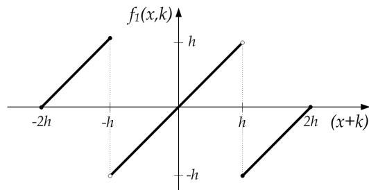
Fig. 13. The graph of non-linear function f_1 .
