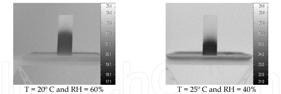
Fig. 8. Thermograms of a cellular concrete specimen after 168 hours of absorption using emissivity 0.85.
