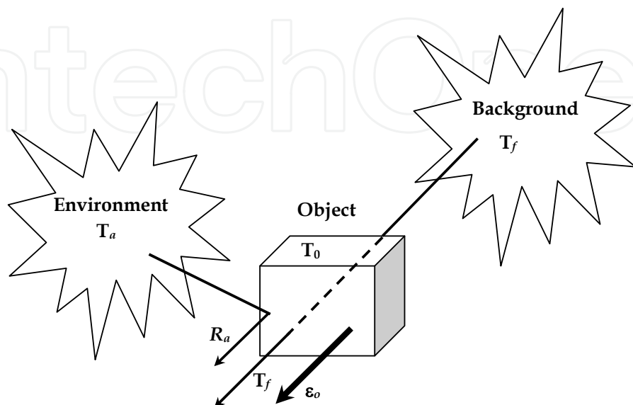
Fig. 6. Factors affecting infrared thermography measurements.
