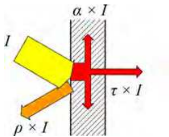
Fig. 5. Radiant energy interacting with a semitransparent surface.
