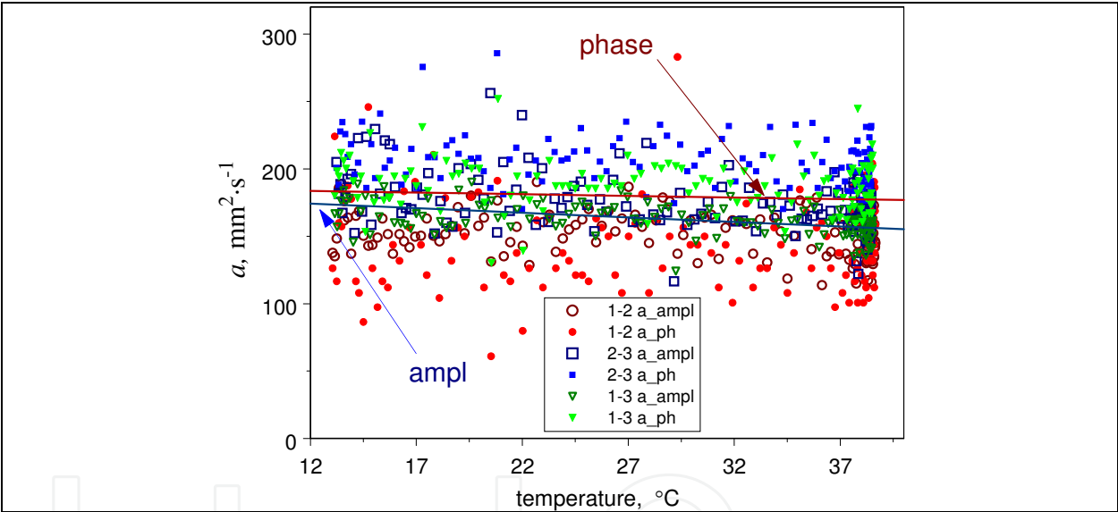
Fig. 10. Results of investigation of the TD temperature dependence of pyrolytic graphite
