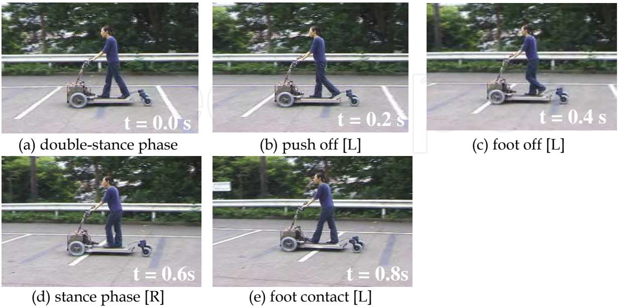
Fig. 12. Gait pattern during walking and driving Tread-Walk1.
