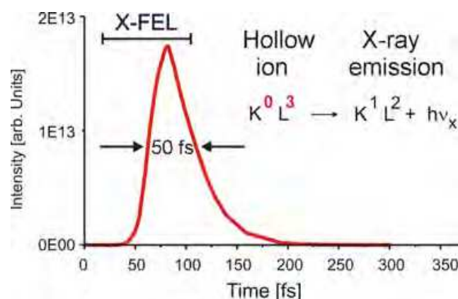
Fig. 4.1. MARIA simulations of the temporal evolution of the hollow ion X-ray emission induced by the interaction of a XFEL pulse with a dense Mg plasma plume, E_{\text{FEL}} = 3100 eV, \tau = 100 fs, \tilde{N}_0 = 10^{23} \text{ cm}^{-3} , I_{\text{max}} = 3.7 \times 10^{17} \text{ W/cm}^2 , n_e = 10^{21} \text{ cm}^{-3} , kT_e = 30 eV.
