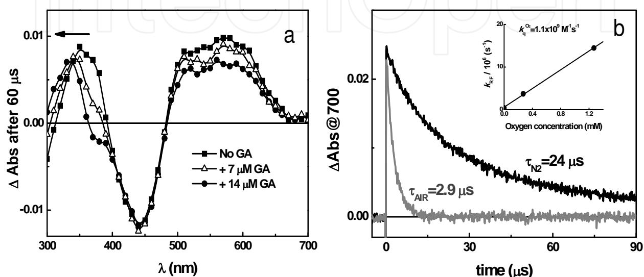
Fig. 2. a) Transient absorption spectra of RF (35 \mu\text{M} ) in \text{N}_2 -saturated MeOH-Water (1:1) solution observed after 60 \mu\text{s} of the laser pulse as a function of the concentration of GA. b) Effect of dissolved molecular oxygen ( ^3\text{O}_2 ) on the decay of the ^3\text{RF}^* at 700 nm. Inset: Stern-Volmer plot for the quenching of ^3\text{RF}^* by ^3\text{O}_2 .
