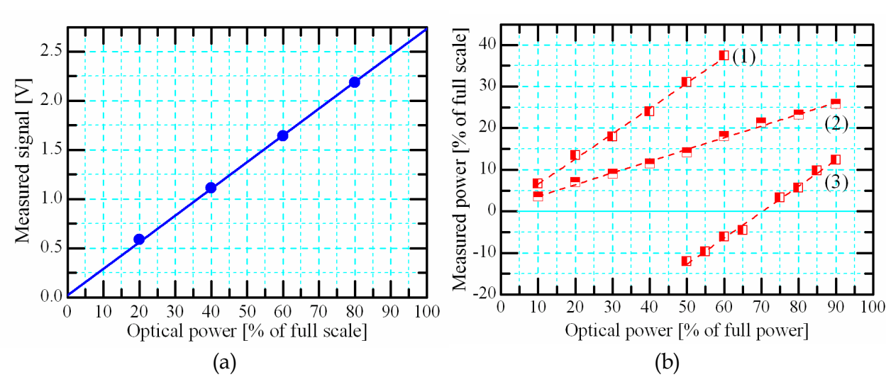
Fig. 17. Transfer functions in open-loop (a) and closed-loop (b). The dashed lines (b) indicate the two different slopes of the transfer functions in closed-loop mode. (1) and (3) exhibit a slope twice as big as the one of (2). (3) is the transfer function in closed-loop mode around 70% optical input power.
