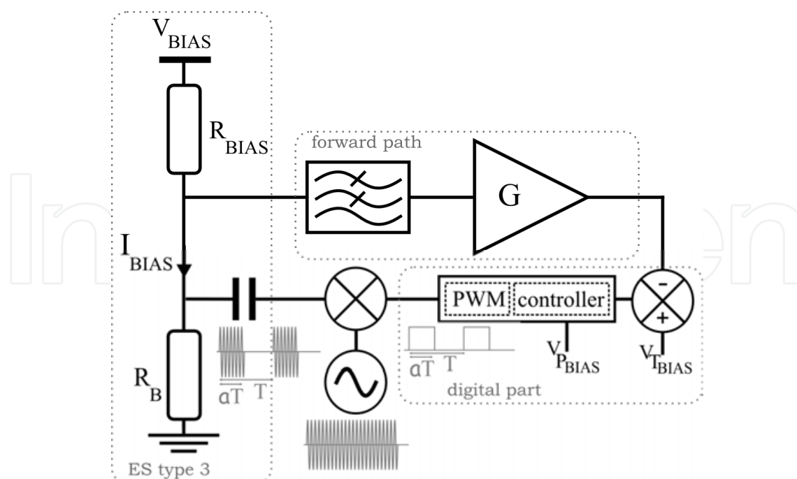
Fig. 8. Schematic of a digital implementation of the capacitively coupled electrical substitution technique for closed-loop operation of a resistive bolometer involving a PWM modulation with a duty cycle a .
