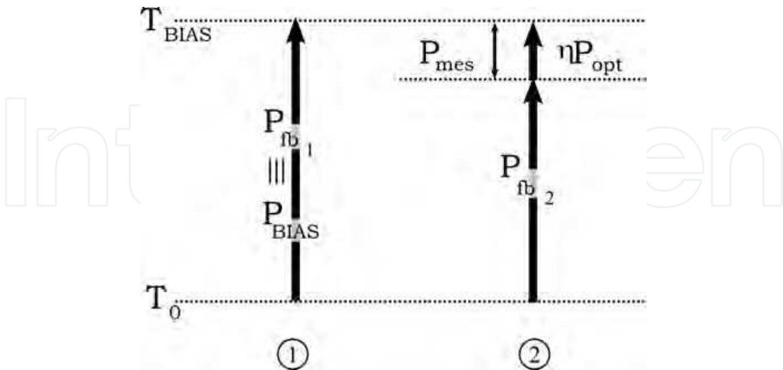
Fig. 7. Electrical substitution principle used for closed-loop mode operation. ① without external optical power, the thermal operating point is set by the bias power corresponding to the V_{P_{bias}} voltage. ② with external optical power, the total amount of power dissipated onto the bolometer is kept constant thanks to the variations of the feedback power.
