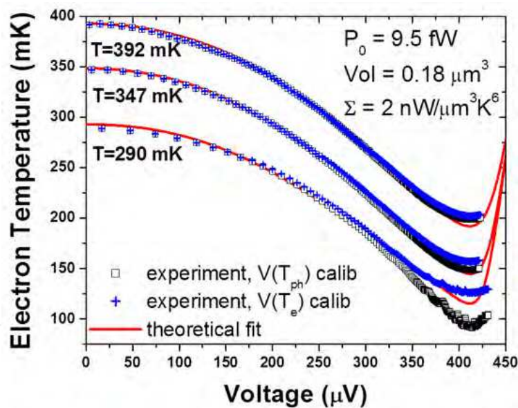
Fig. 20. Electron temperature measured for phonon temperatures of 392 mK, 347 mK and 290 mK. Theoretical fit for background power of 9.5 fW, absorber volume 0.18 \mu m 3 .
