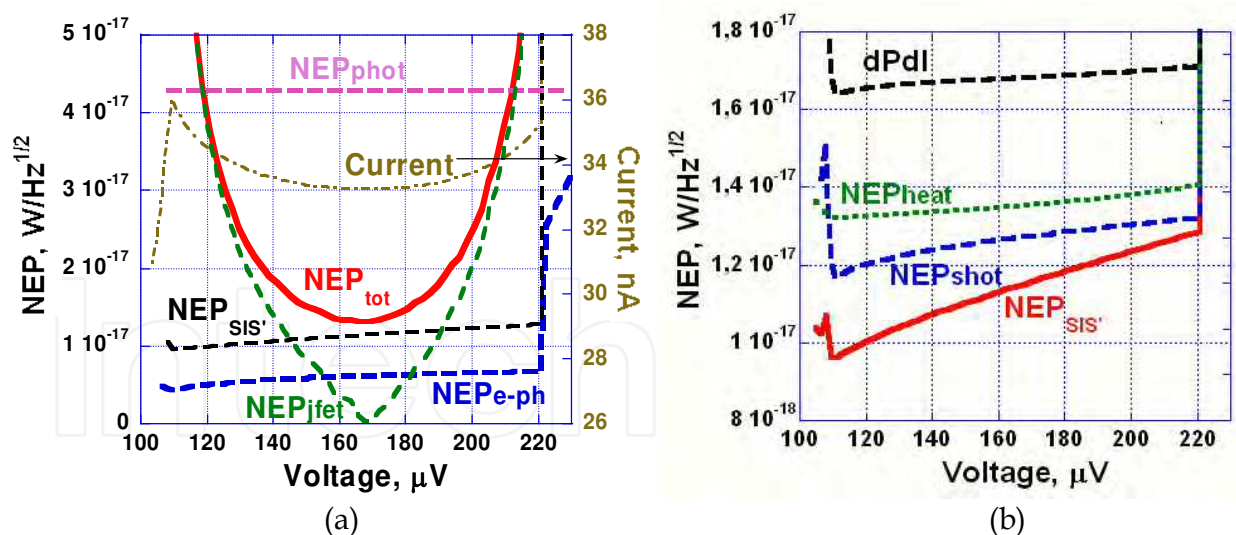
Fig. 15. (a) NEP components of the SCEB for I_{JFET}=5 \text{ fA/Hz}^{1/2} , V_{JFET}=3 \text{ nV/Hz}^{1/2} , R=0.2 \text{ kOhm} , A=0.04 \mu\text{m}^3 . The NEP_{tot} is less than NEP_{phot} ; (b) Resulting SIS' junction noise with strong cancellation of the NEP_{shot} and NEP_{heat} due to the anticorrelation term dPdI between them.
