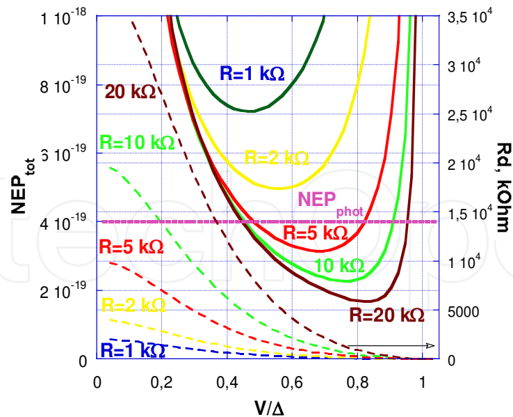
Fig. 13. NEP components of the 2D array of CEBs with the JFET readout at 7 THz with power load of 0.02 fW for I_{JFET}=5 \text{ fA/Hz}^{1/2} , V_{JFET}=3 \text{ nV/Hz}^{1/2} , \Delta=0.002 \mu\text{m}^3 , T=70 \text{ mK} , T_c=400 \text{ mK} for different values of normal resistance R .
