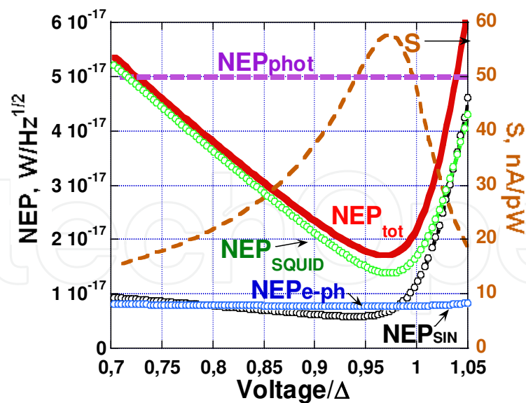
Fig. 17. Total NEP of the 40 CEB array with SIN tunnel junctions for the 350 GHz channel, with a SQUID noise current of 0.8 pA/Hz 1/2 . Parameters: R=0.2 kOhm, S=1\mu\text{m}^2 , \text{Vol}=0.005\mu\text{m}^3 , power load P_0 = 5 pW, T=300 mK. The \text{NEP}_{\text{phot}}= 5\cdot 10^{-17} W/Hz 1/2 is shown by dashed line.per polarization component. For the 70GHz channel, \text{NEP}_{\text{phot}}= 4.3\cdot 10^{-18} W/Hz 1/2 .
