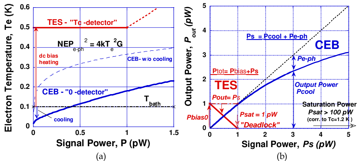
Fig. 2. (a) Electron temperature as a function of signal power for T_{\text{bath}}=100\text{ mK} for CEB and TES. For CEB, the T_e is always cooled to the lowest possible level. For P<0.4\text{ pW} , the T_e of CEB is less than T_{\text{bath}} (real cold-electron bolometer). For TES, the T_e is equal to T_c for all range of operation up to saturation power. After saturation there is uncontrollable increase of temperature. (b) Output power (cooling power) of the CEB in dependence on signal power (blue). They are almost equal at a small level of power. At a higher level of power, the P is split between P_{\text{cool}} and P_{e-ph} . The saturation power would be achieved only after heating to T_c of Al electrode ( P_{\text{sat}} is around 100 pW). Bias power and output power of the TES on signal power (red). Saturation power is equal to the full bias power at zero signal.
